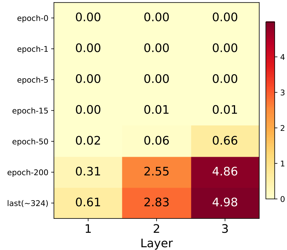
RMSE vs 0
