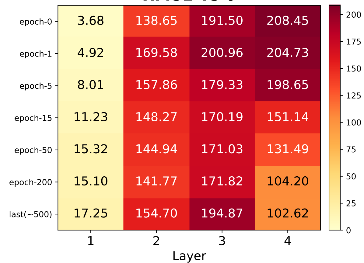
RMSE vs 0
