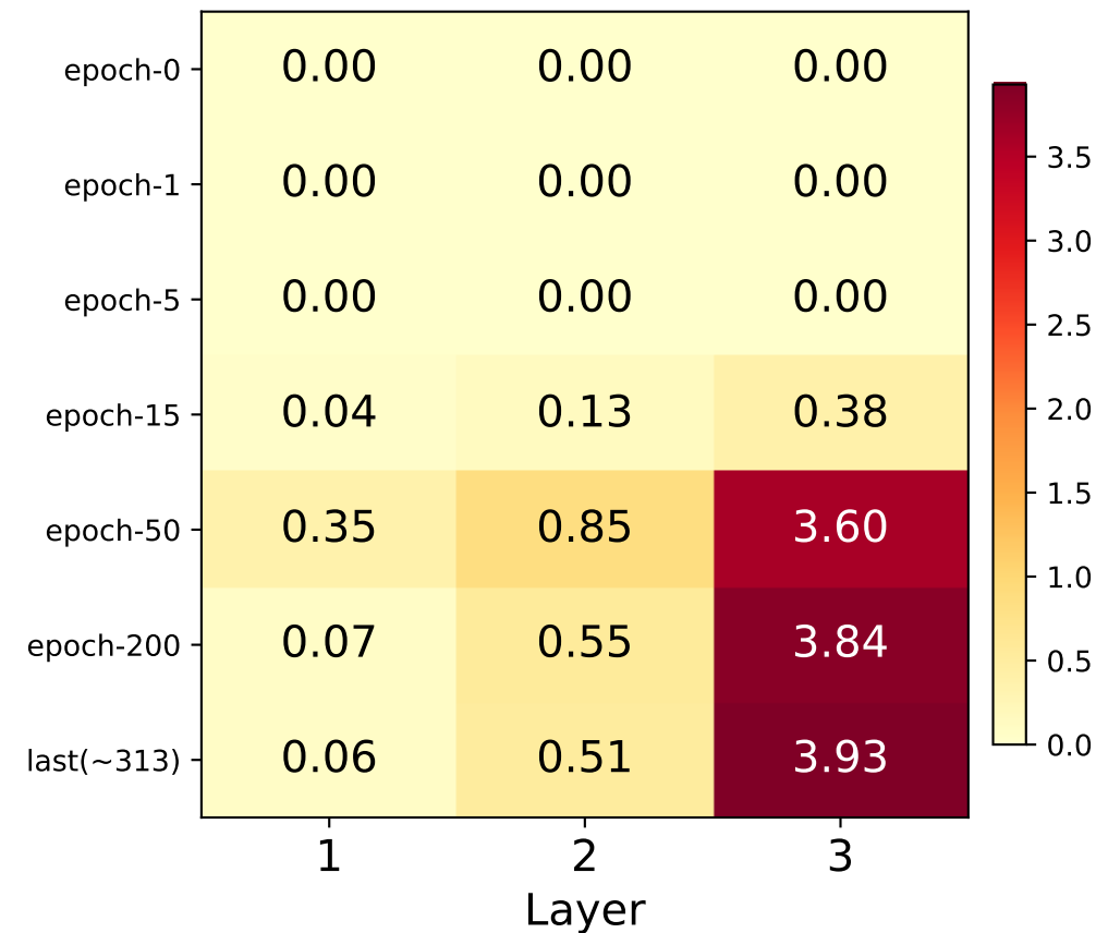
RMSE vs 0
