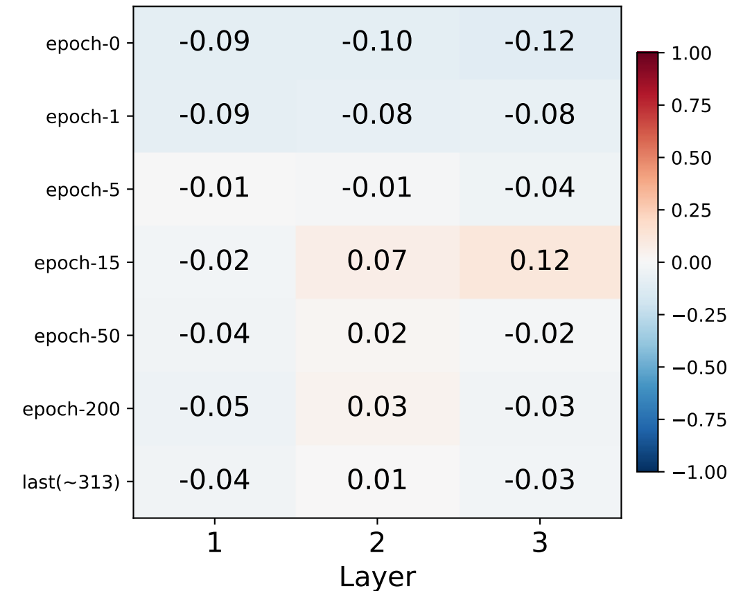
RMSE vs 0
