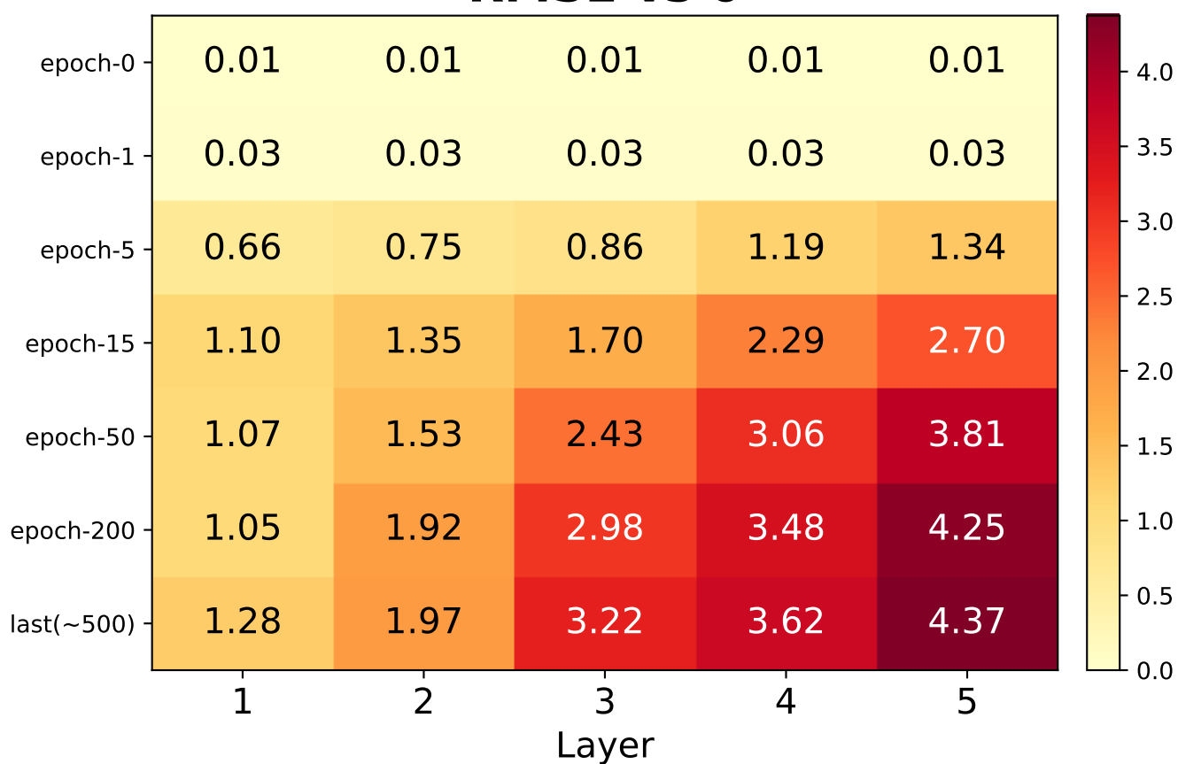
RMSE vs 0
