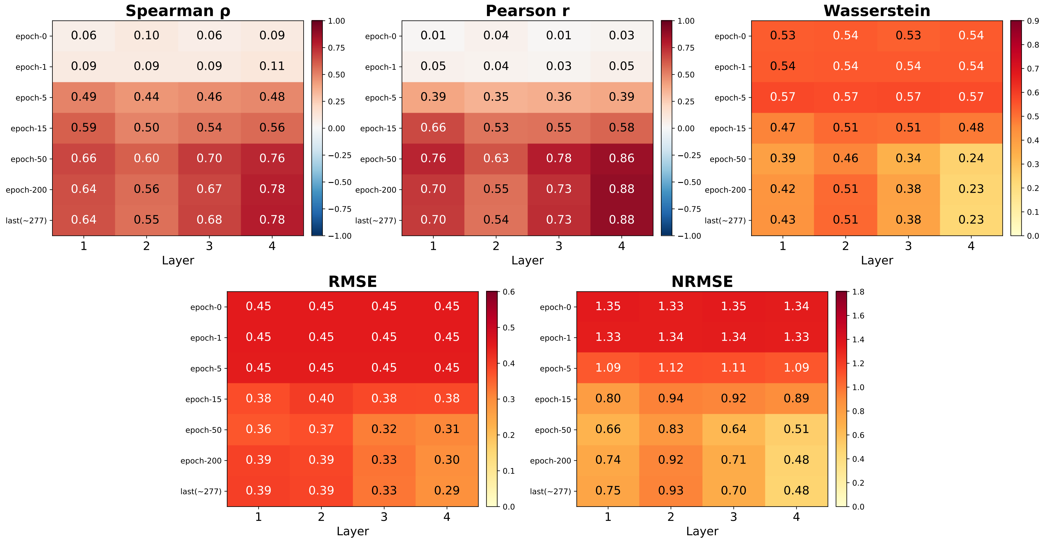
Forman Alignment Heatmap — pubmed (GeneralSheaf, d=5, 4L, norm=True) (values = mean across 5 eigenvalues, averaged over folds)
