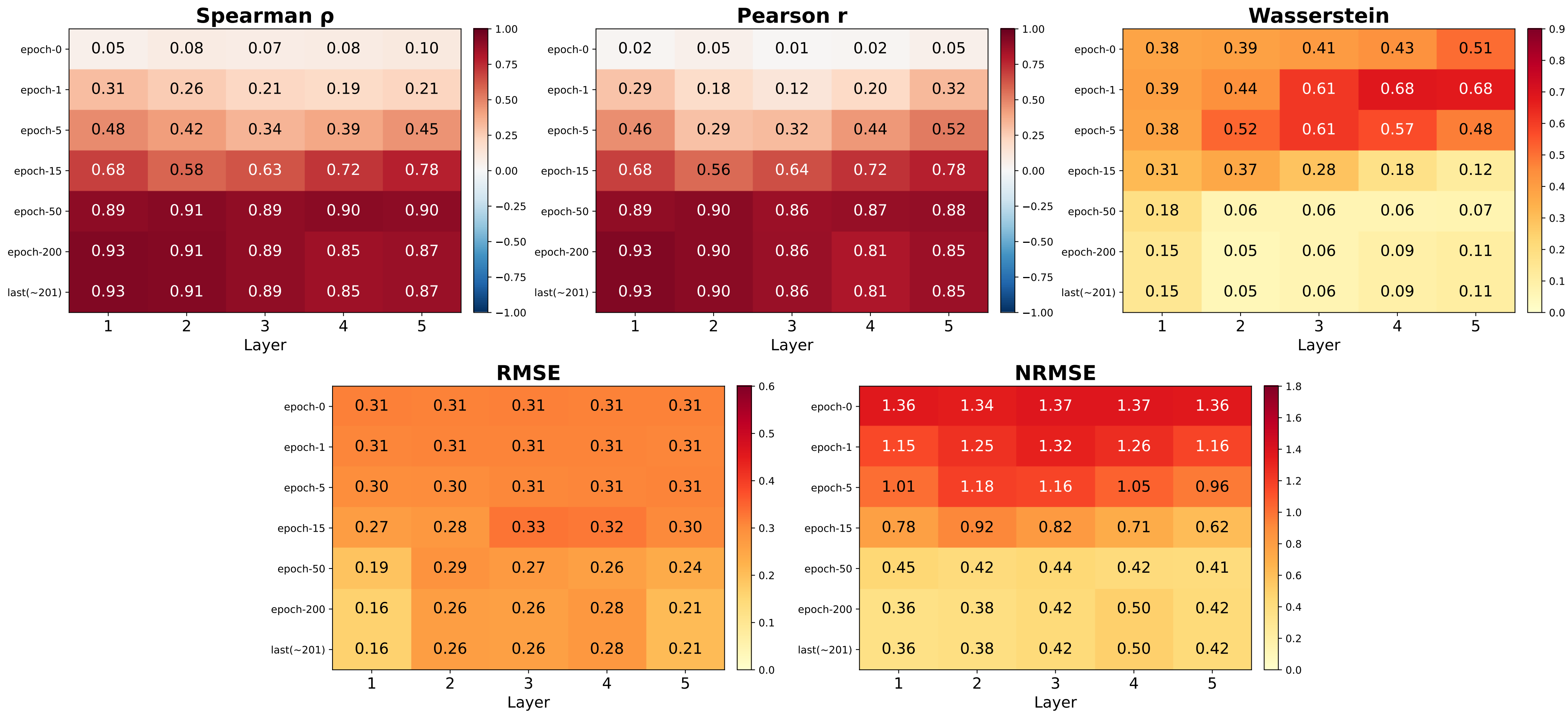
Forman Alignment Heatmap — amazon_ratings (GeneralSheaf, d=5, 5L, norm=False) (values = mean across 5 eigenvalues, averaged over folds)
