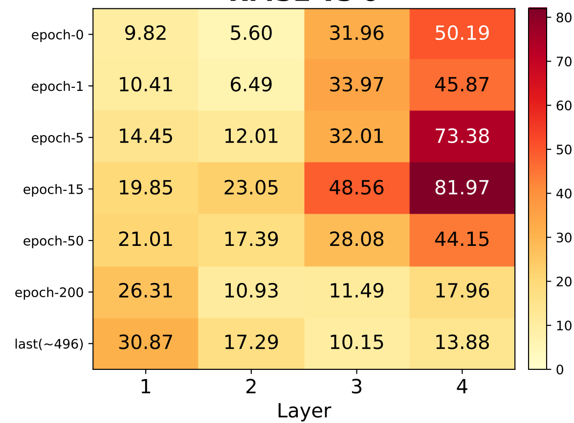
RMSE vs 0
