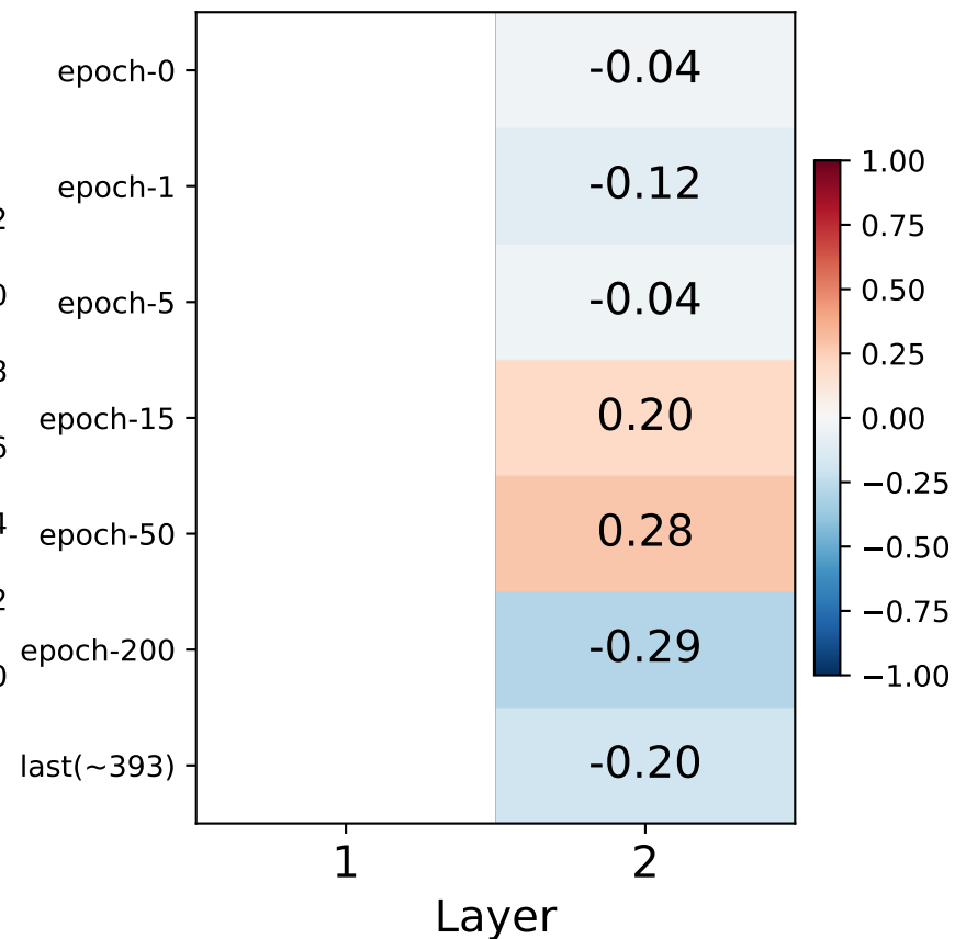
RMSE vs 0
