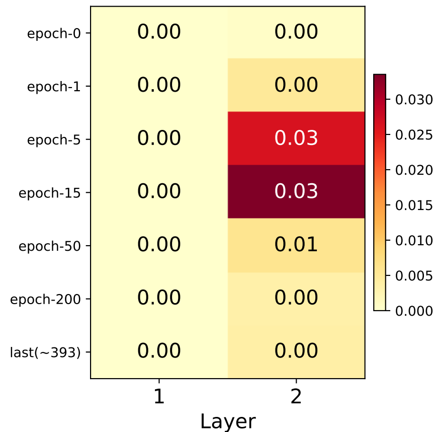
RMSE vs 0
