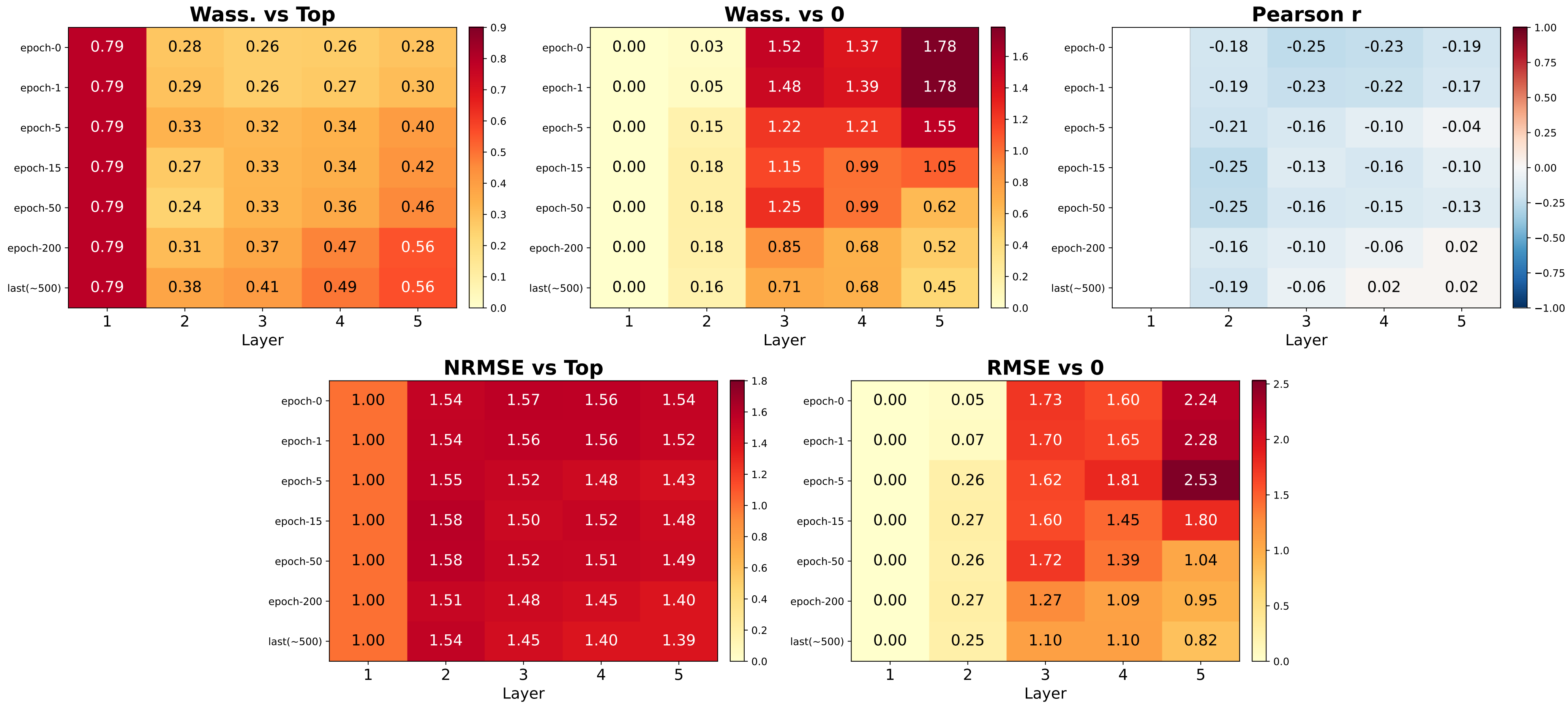
Forman Alignment Heatmap — roman_empire (JointSheafParams, d=5, 5L, norm=False) (values = mean across 5 eigenvalues, averaged over folds)
