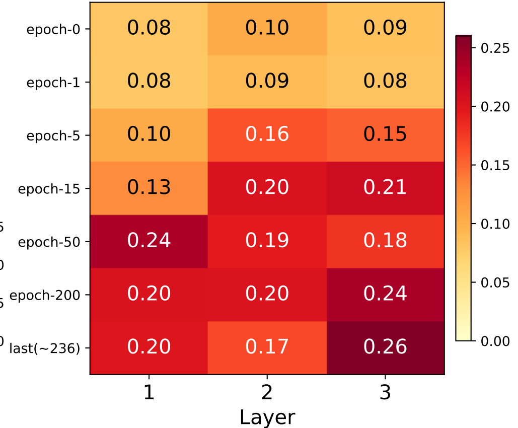
NRMSE
