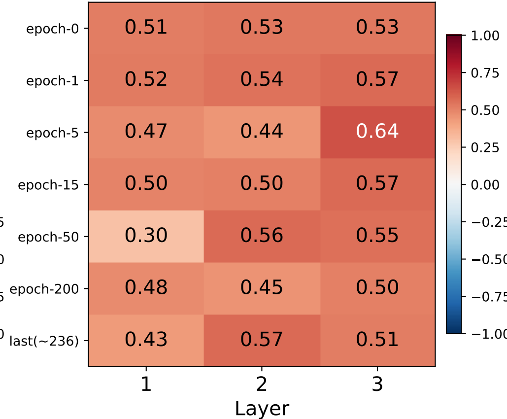
RMSE
