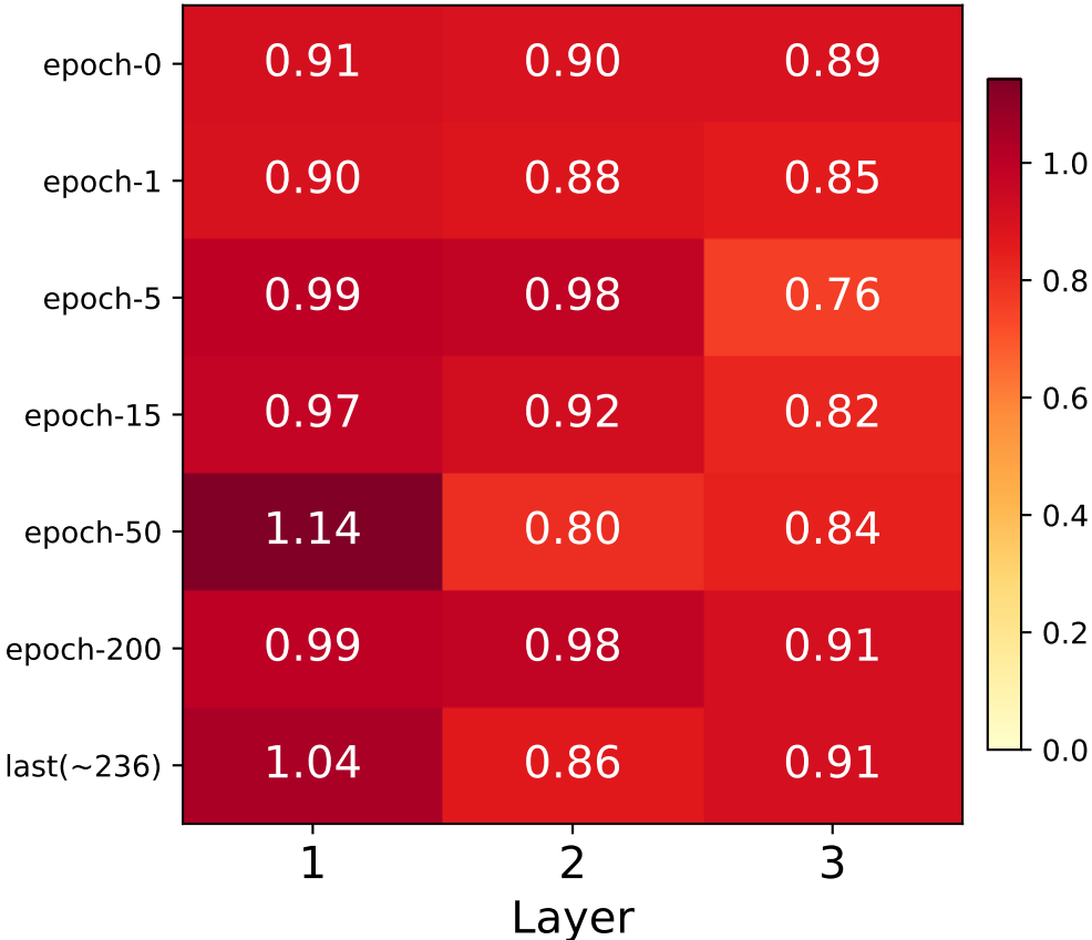
NRMSE
