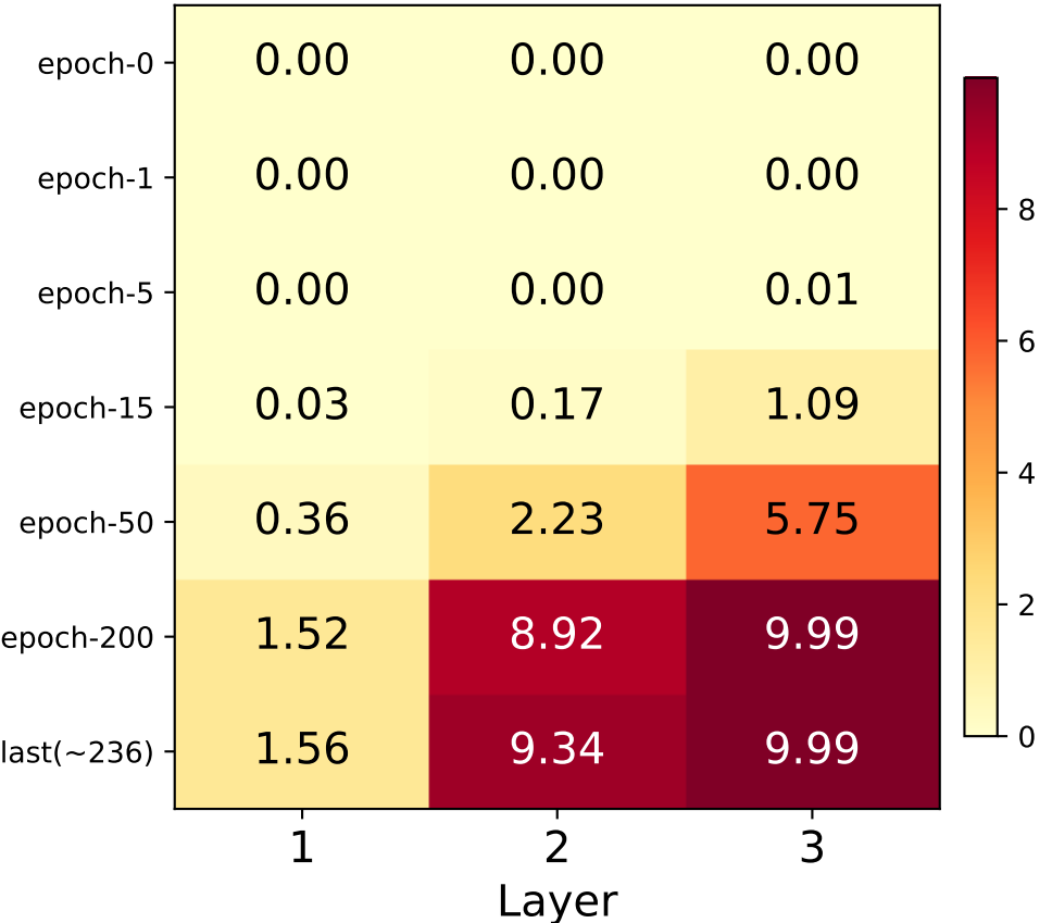
RMSE
