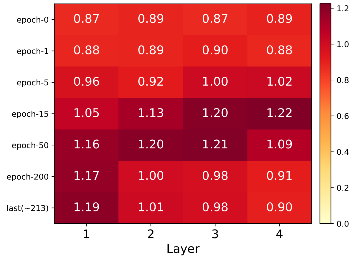
NRMSE
