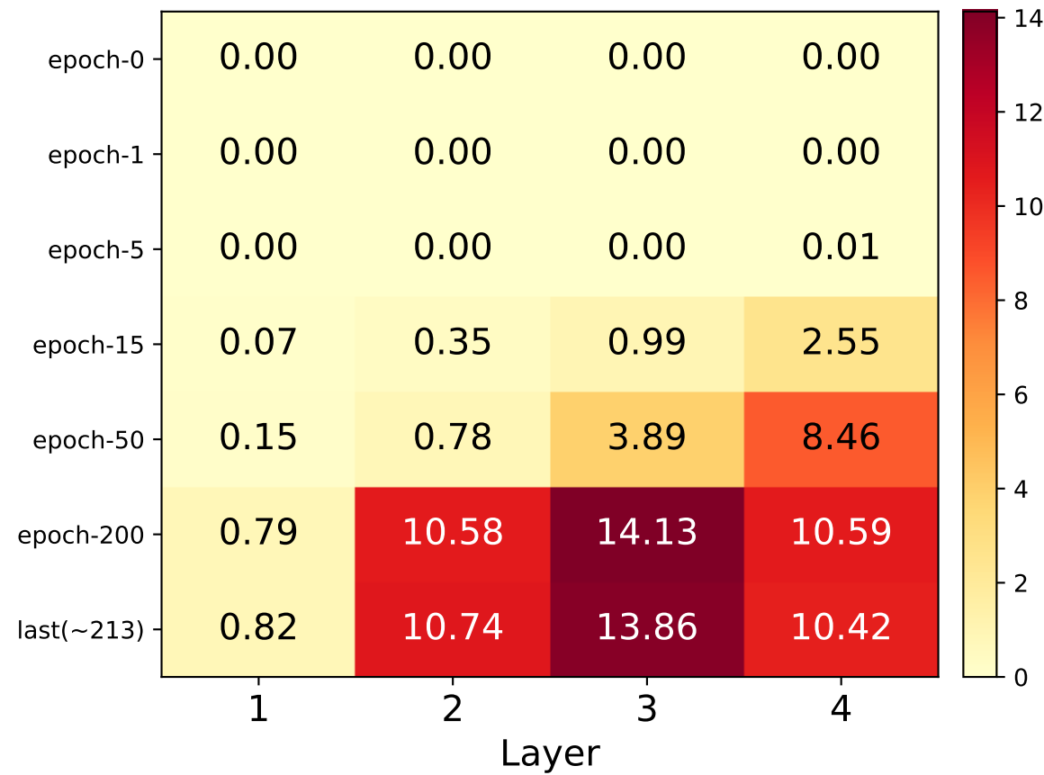
RMSE
