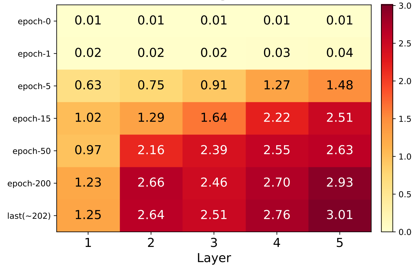
RMSE
