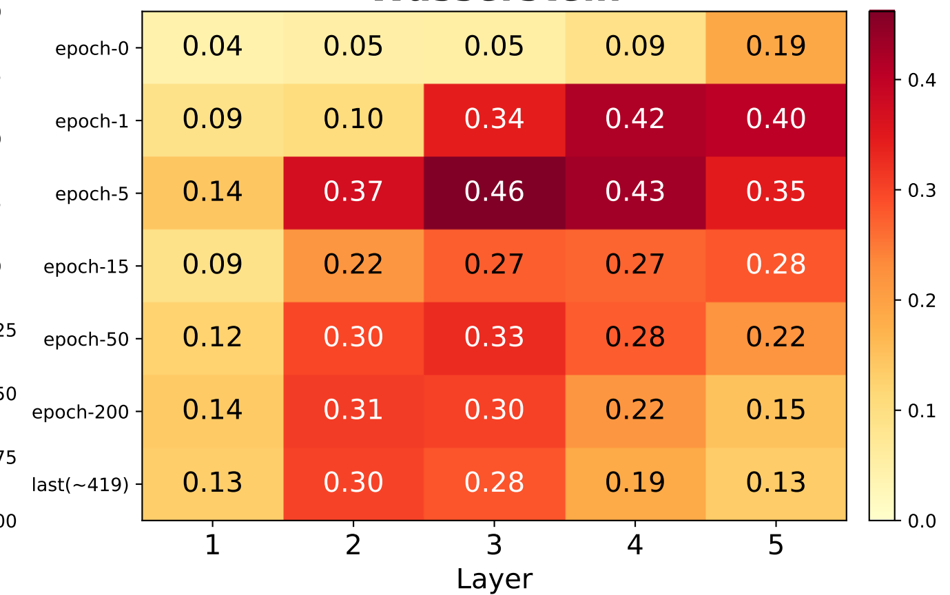
NRMSE
