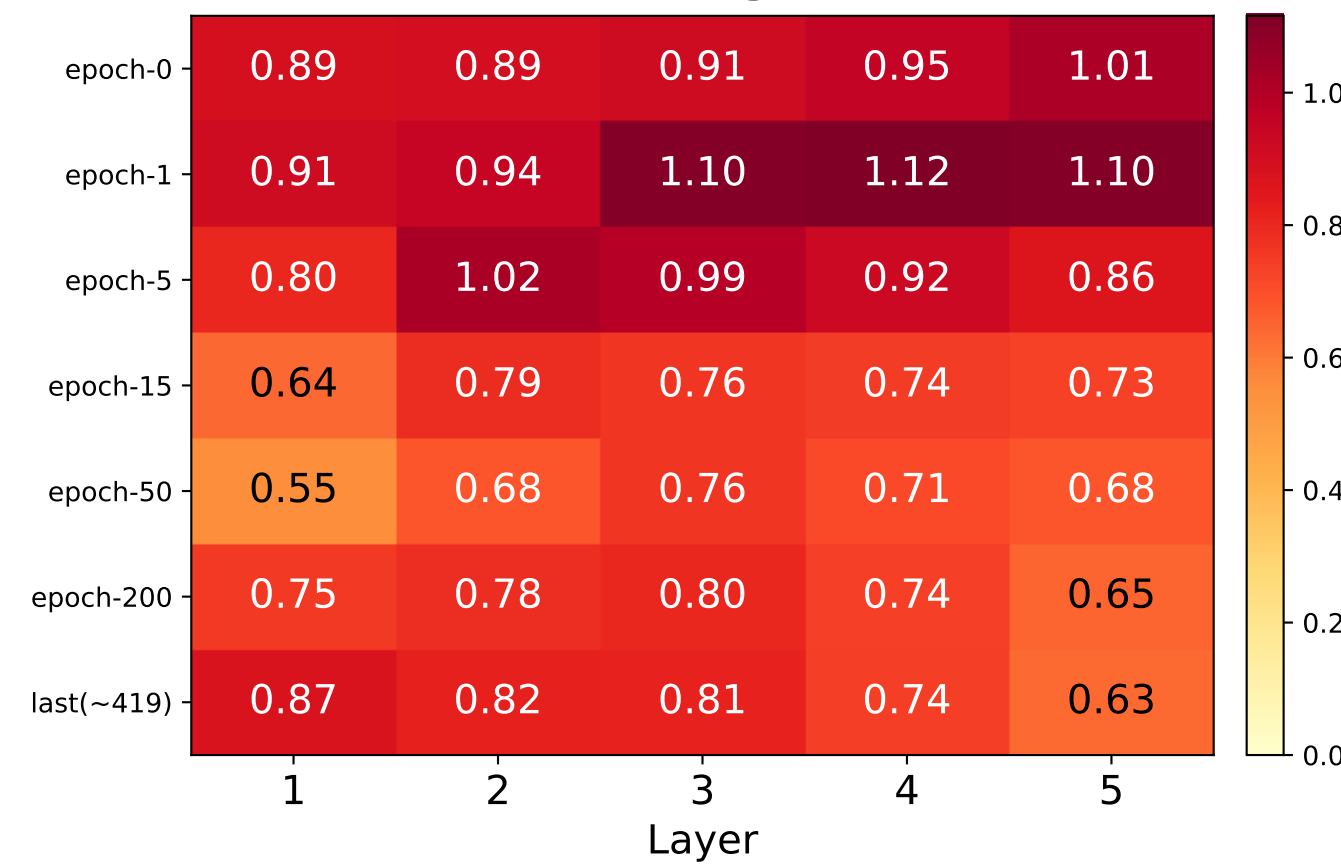
NRMSE
