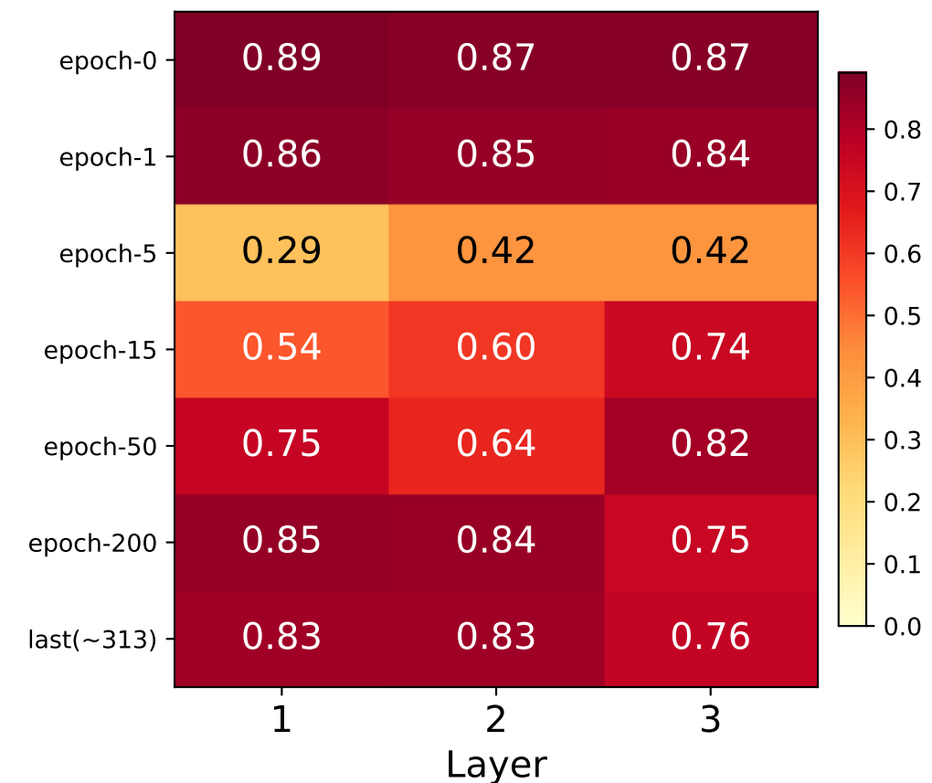
NRMSE
