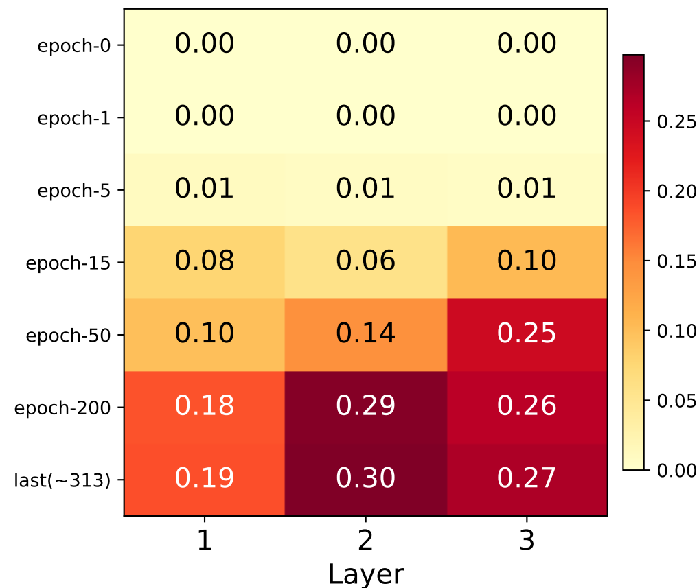
RMSE
