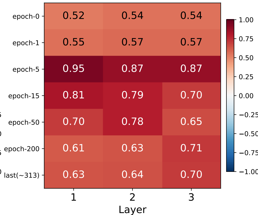
RMSE
