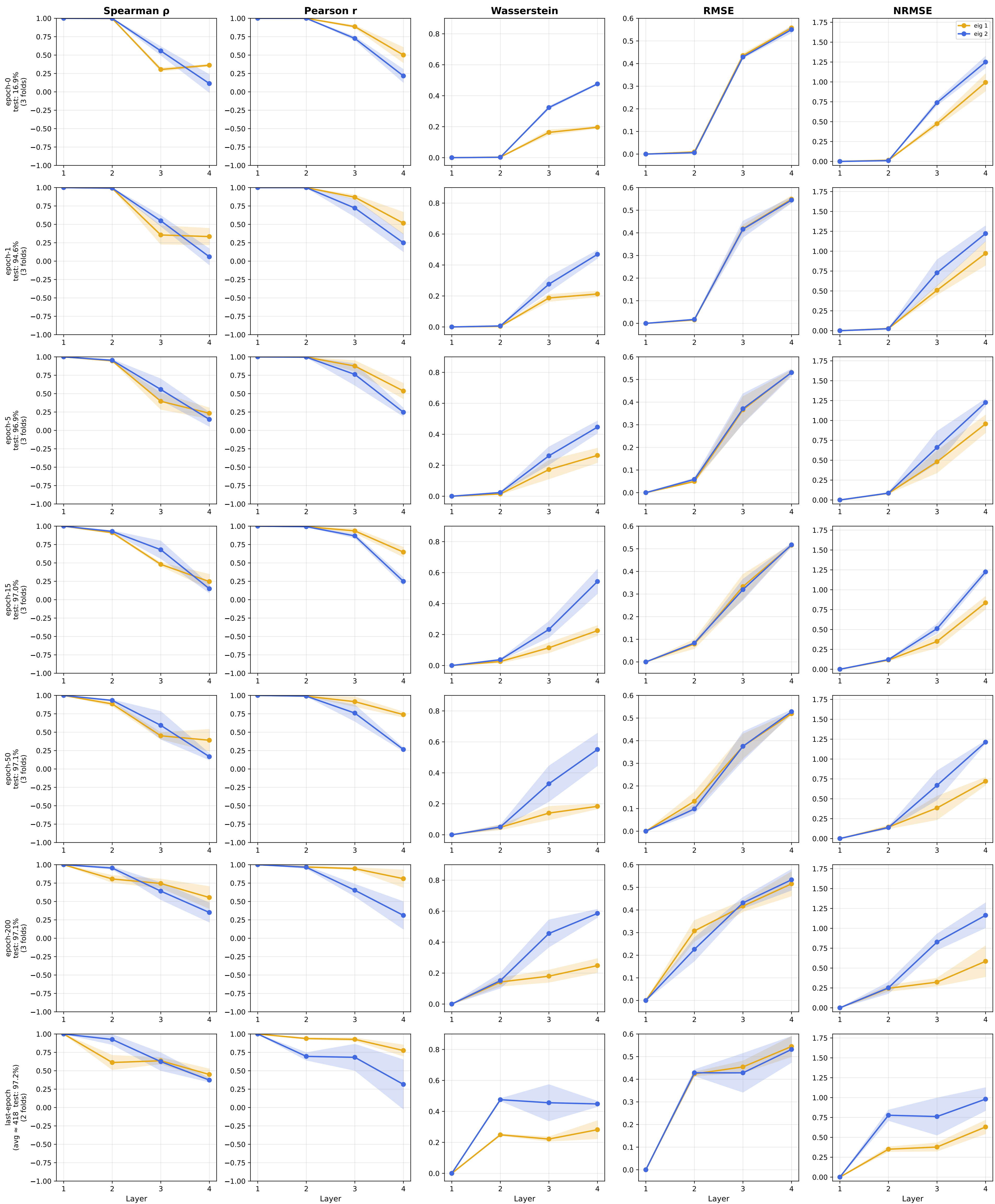
Forman Profile Evolution — questions (JointSheafParams, d=2, 4L, norm=True)
