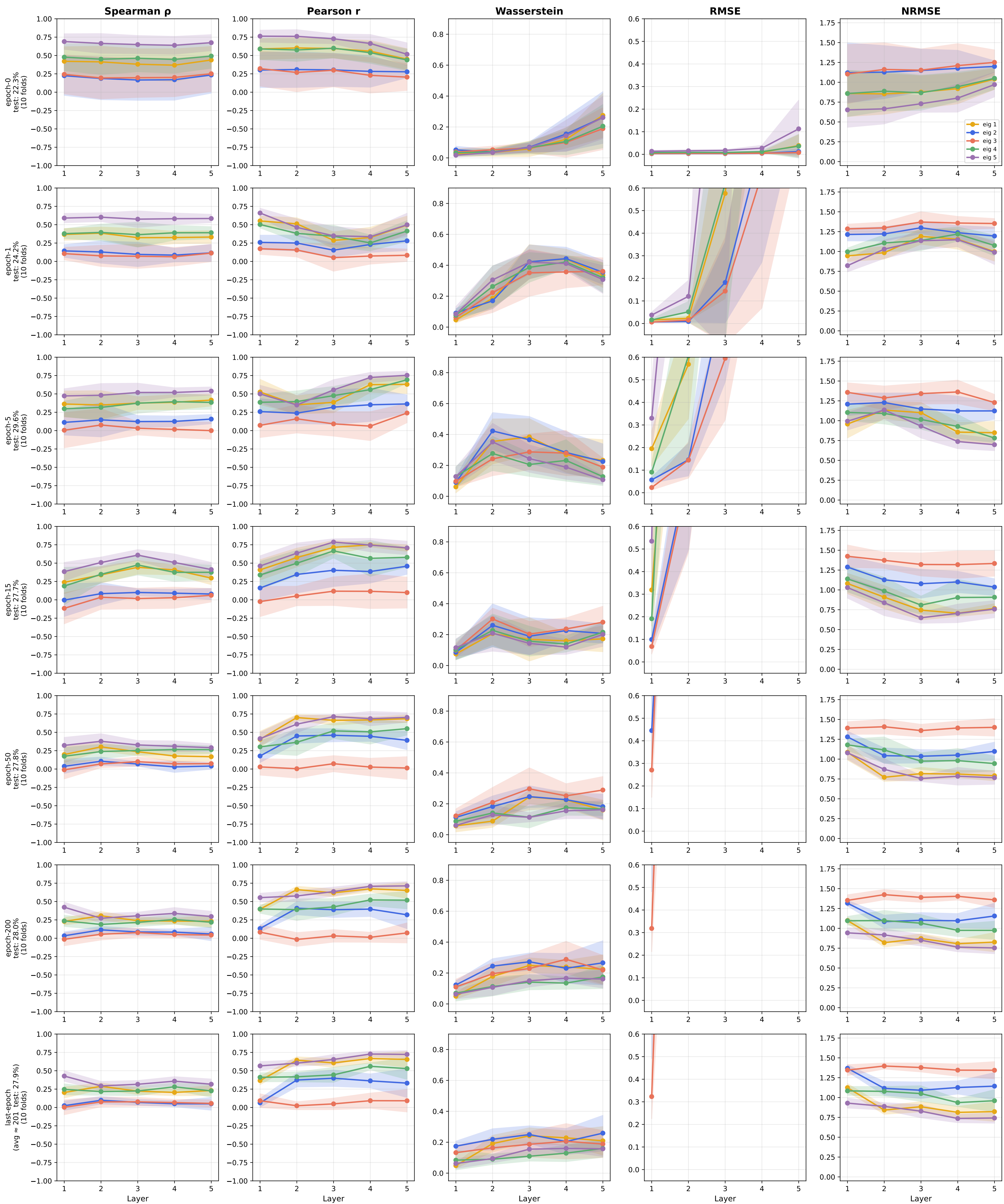
Forman Cross-Comparison — amazon_ratings (GeneralSheaf, d=5, 5L) Trained norm=False → unnorm. LaplacianF (primary) vs Trained norm=True → unnorm. LaplacianF (via other_Laplacian)
