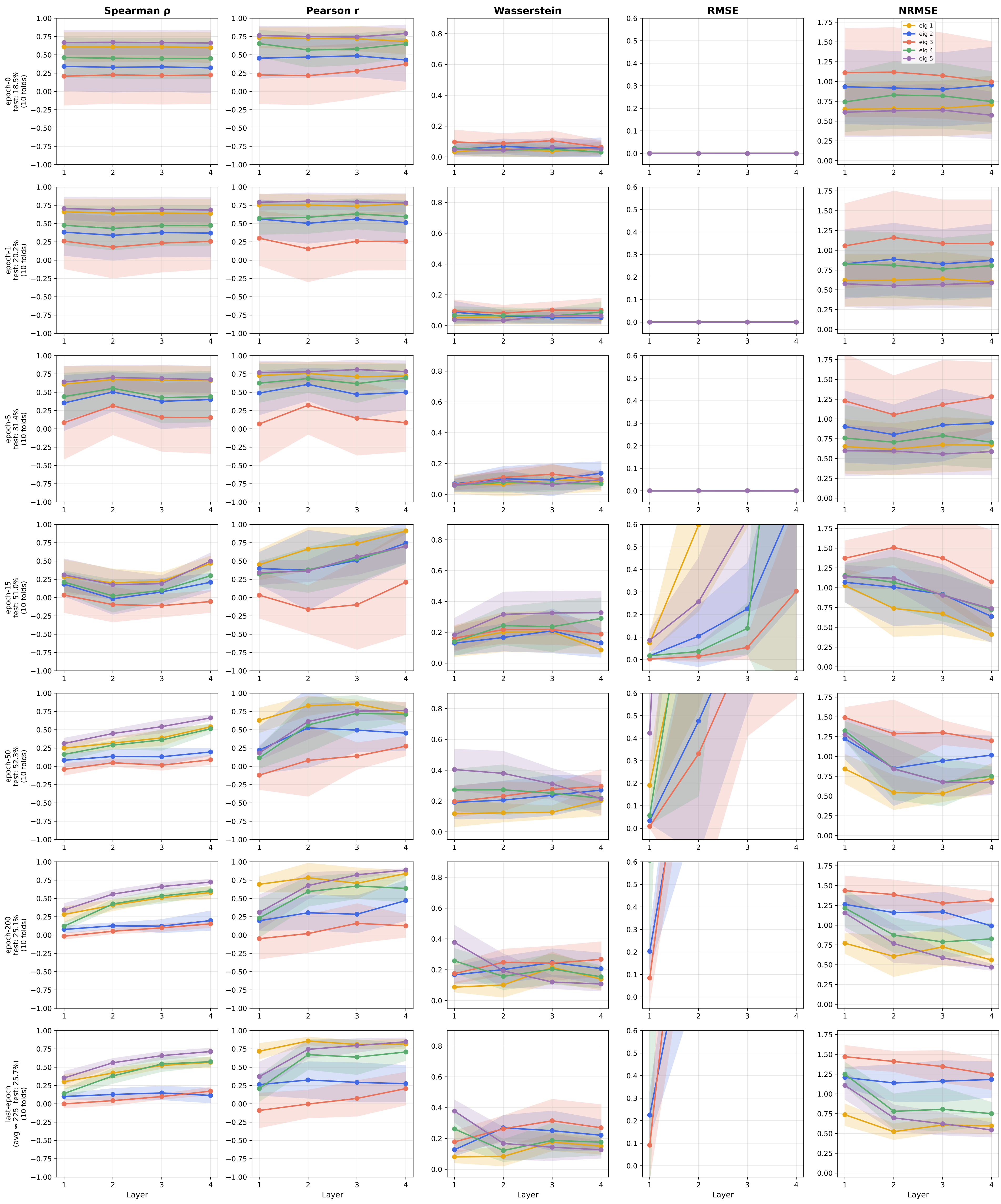
Forman Cross-Comparison — citeseer (GeneralSheaf, d=5, 4L) Trained norm=False → unnorm. LaplacianF (primary) vs Trained norm=True → unnorm. LaplacianF (via other_Laplacian)
