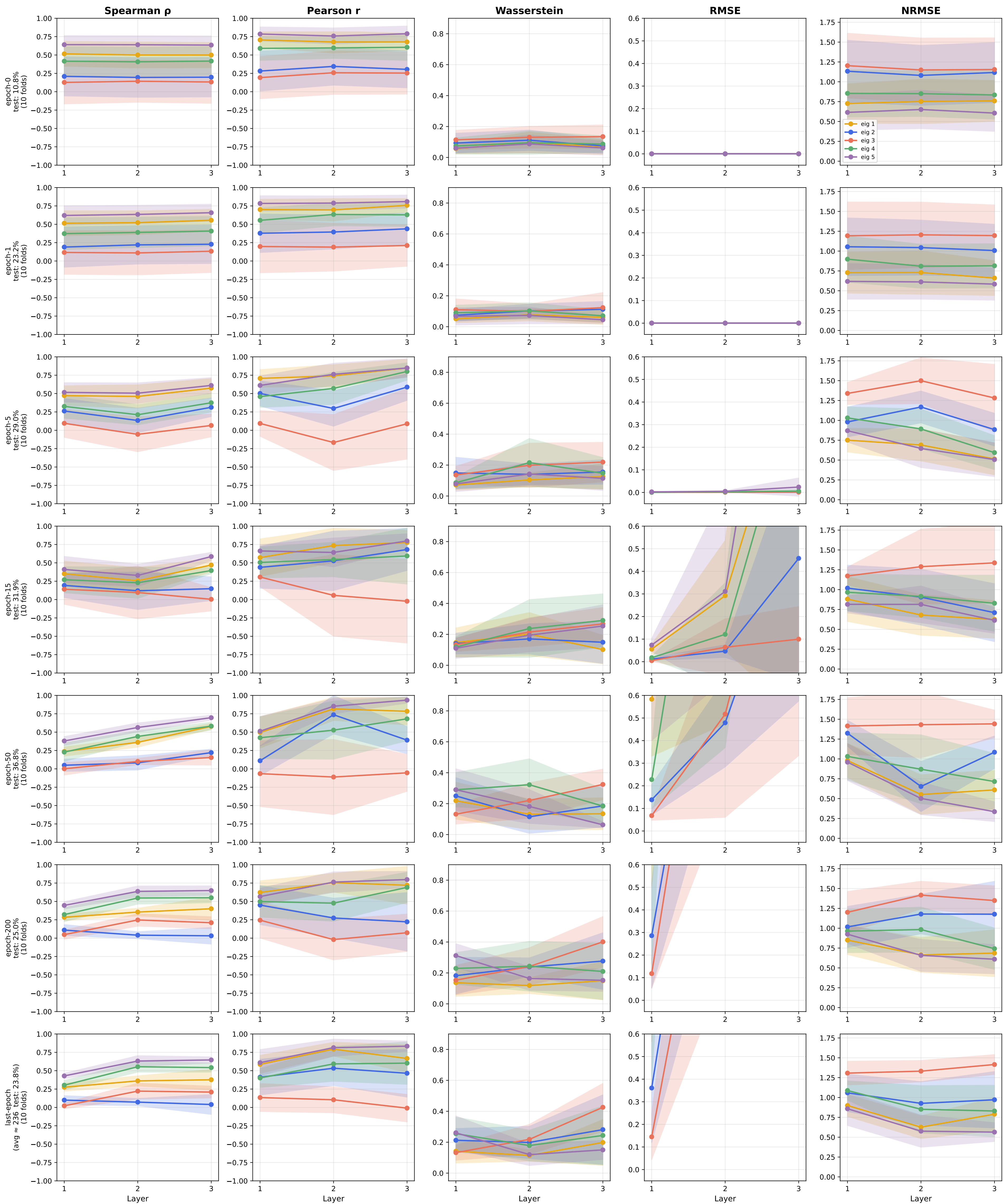
Forman Cross-Comparison — cora (GeneralSheaf, d=5, 3L) Trained norm=False → unnorm. LaplacianF (primary) vs Trained norm=True → unnorm. LaplacianF (via other_Laplacian)
