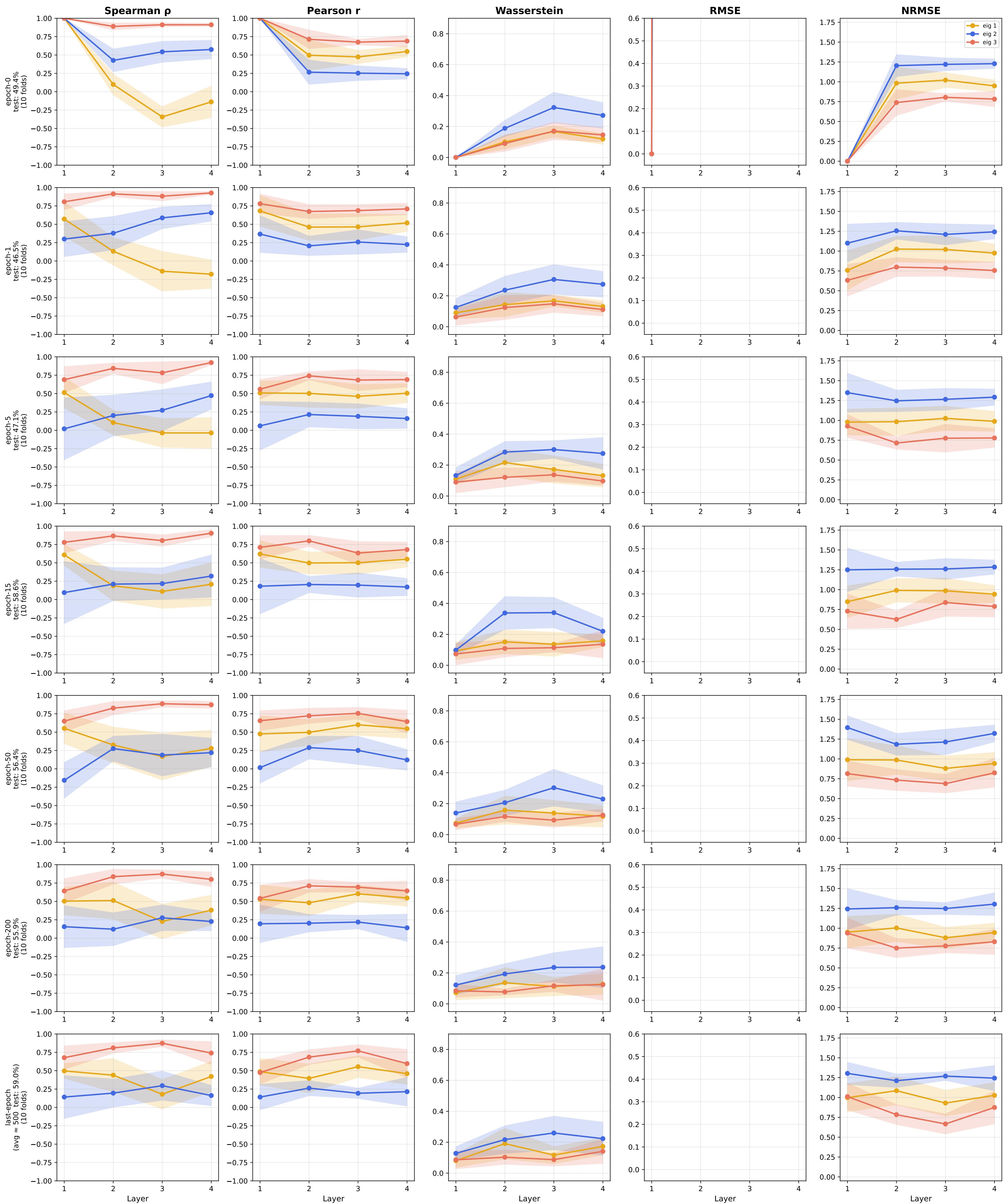
Forman Cross-Comparison — tolokers (GeneralSheaf, d=3, 4L) Trained norm=False → unnorm. LaplacianF (primary) vs Trained norm=True → unnorm. LaplacianF (via other_Laplacian)
