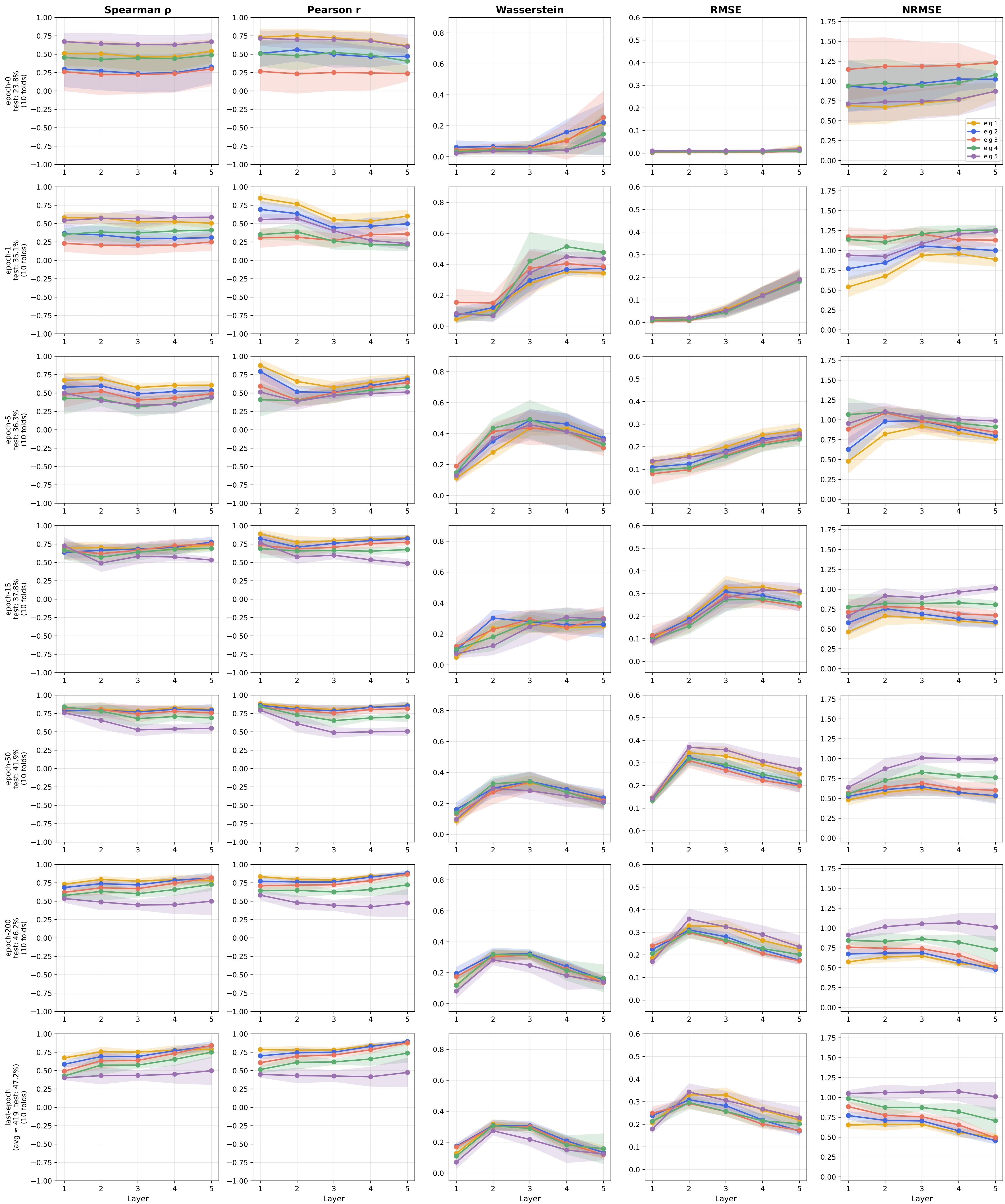
Forman Cross-Comparison — amazon_ratings (GeneralSheaf, d=5, 5L) Trained norm=True → normalised LaplacianF (primary) vs Trained norm=False → normalised LaplacianF (via other_Laplacian)
