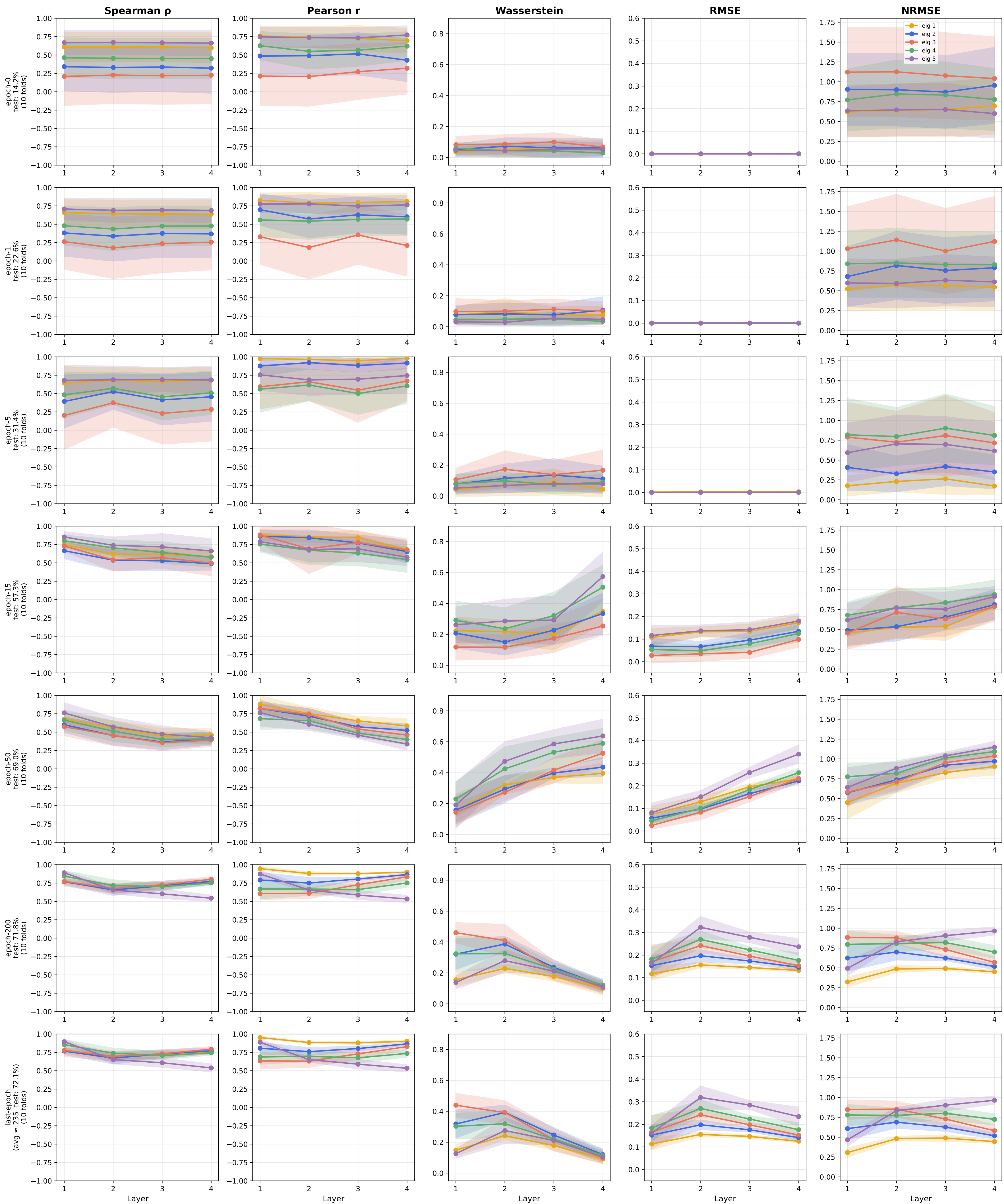
Forman Cross-Comparison — citeseer (GeneralSheaf, d=5, 4L) Trained norm=True → normalised LaplacianF (primary) vs Trained norm=False → normalised LaplacianF (via other_Laplacian)
