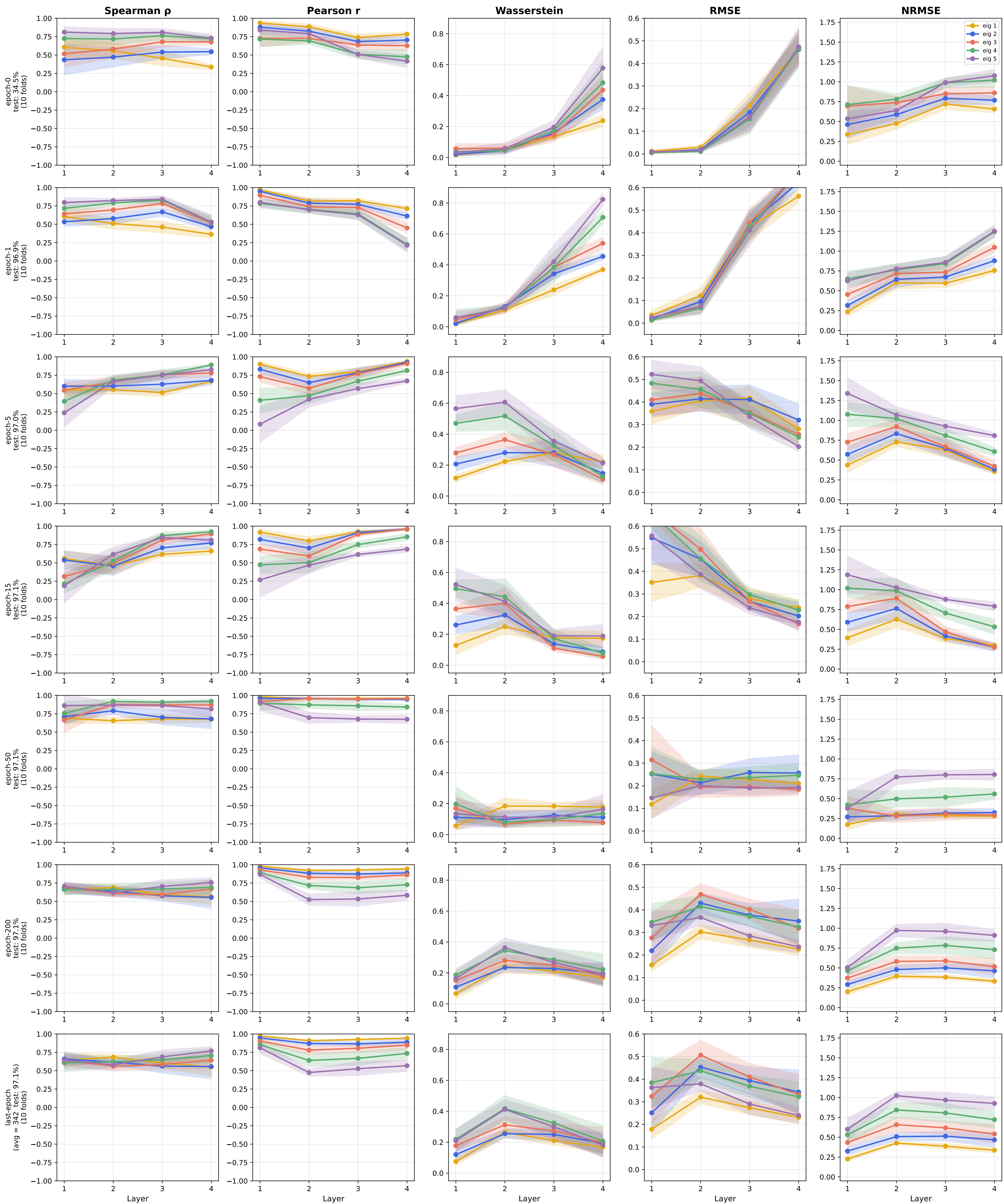
Forman Cross-Comparison — questions (GeneralSheaf, d=5, 4L) Trained norm=True → normalised LaplacianF (primary) vs Trained norm=False → normalised LaplacianF (via other_Laplacian)
