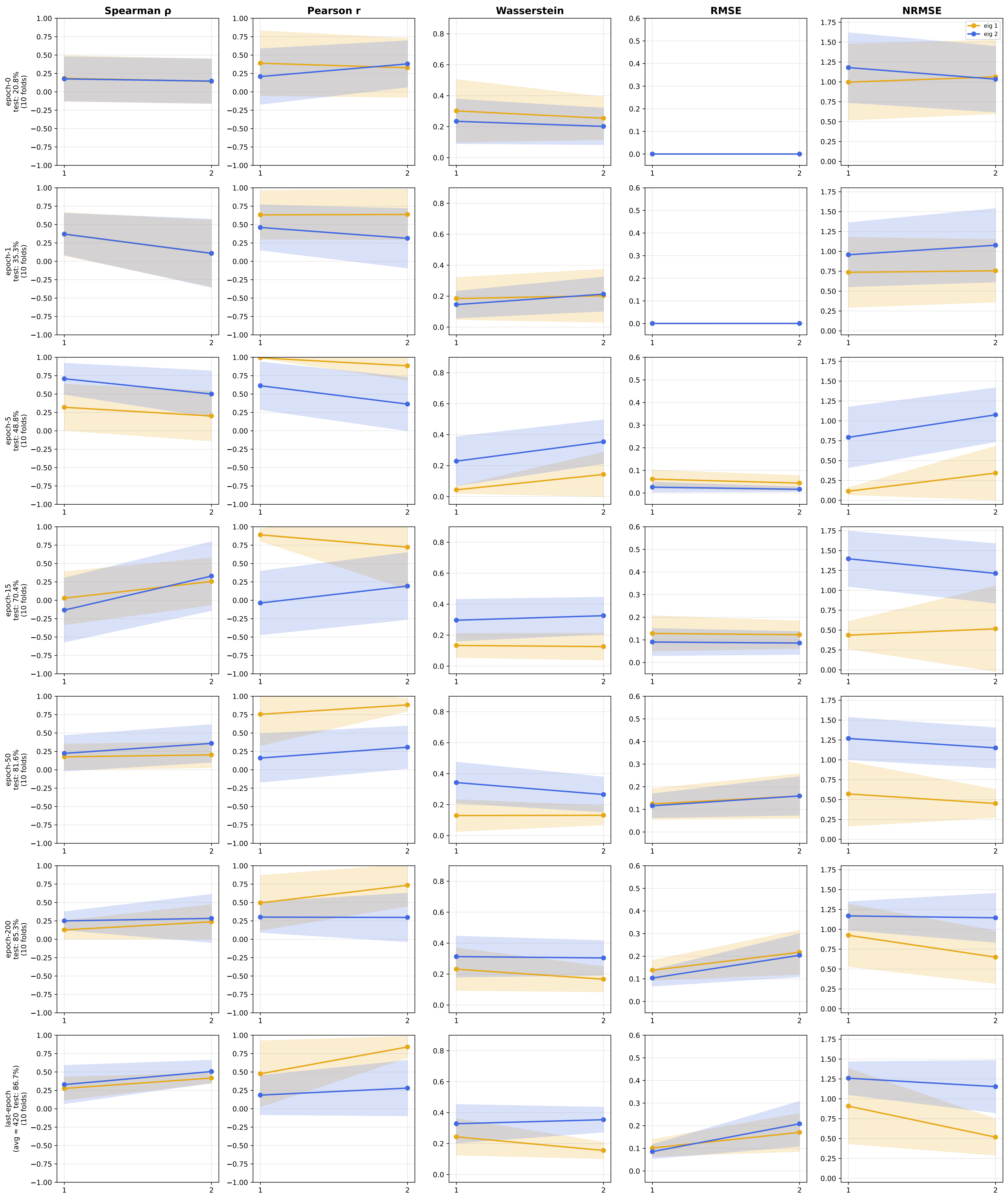
Forman Cross-Comparison — wisconsin (GeneralSheaf, d=2, 2L) Trained norm=True → normalised LaplacianF (primary) vs Trained norm=False → normalised LaplacianF (via other_Laplacian)
