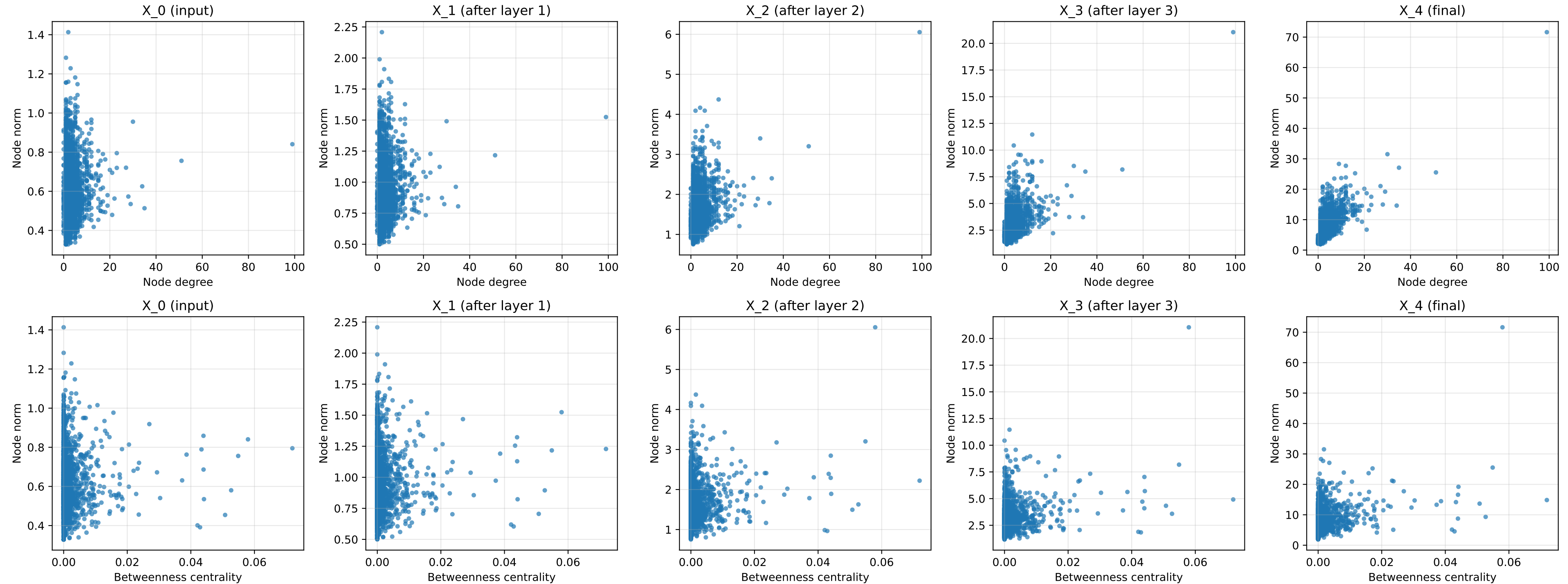
Node norm vs degree / betweenness — citeseer, GeneralSheaf, stalk_dim=5
