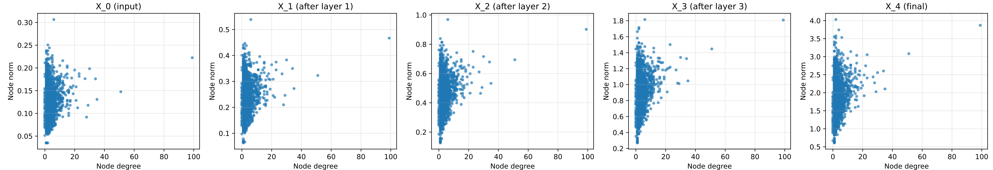
Node norm vs degree — citeseer, JointSheafParamsAlt, stalk_dim=5
