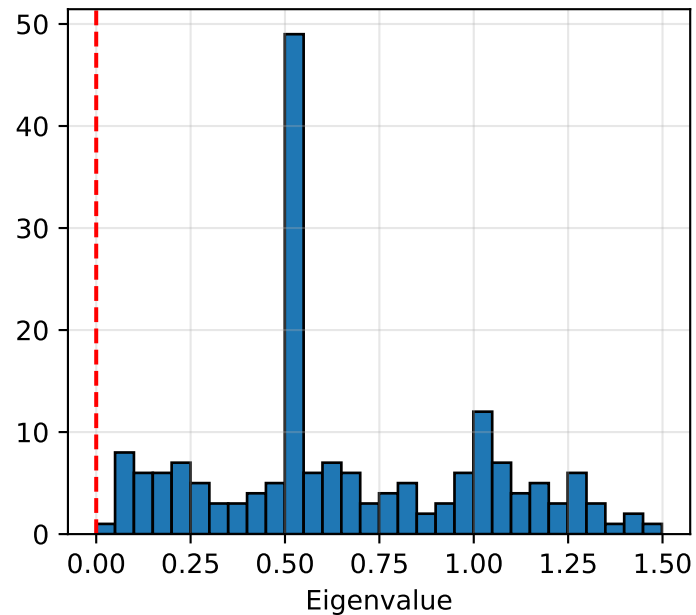
Topological Laplacian
