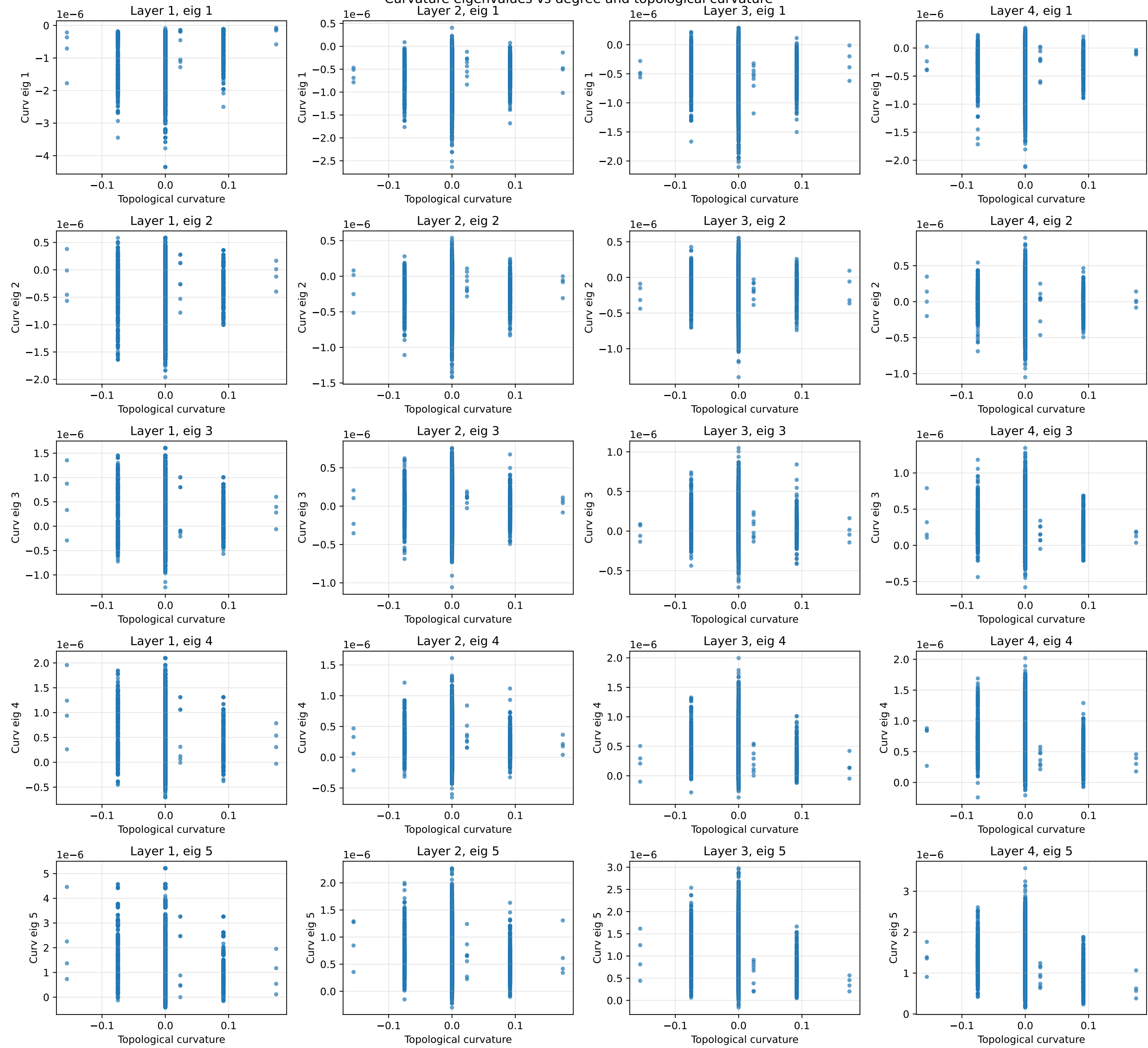
Curvature eigenvalues vs degree and topological curvature
