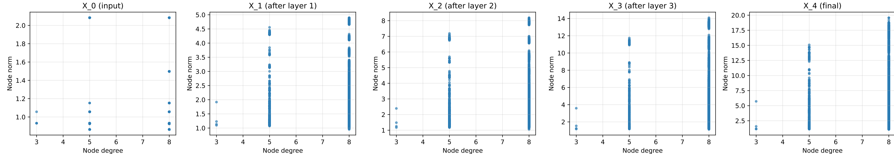
Node norm vs degree — minesweeper, BundleSheaf, stalk_dim=5
