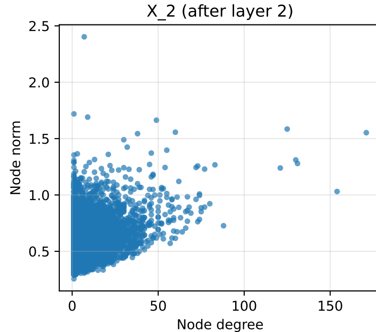
Node norm vs degree — pubmed, GeneralSheaf, stalk_dim=5
