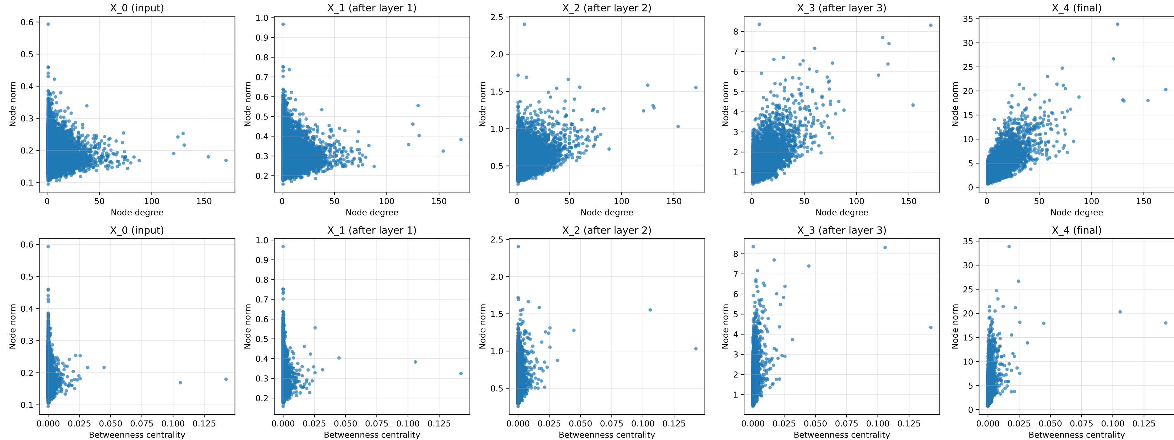
Node norm vs degree / betweenness — pubmed, GeneralSheaf, stalk_dim=5
