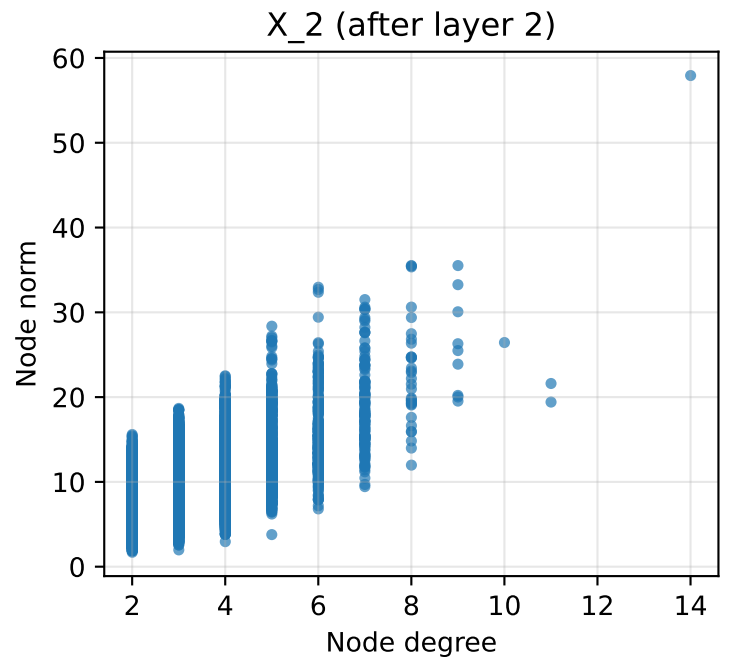
Node norm vs degree — roman_empire, BundleSheaf, stalk_dim=5
