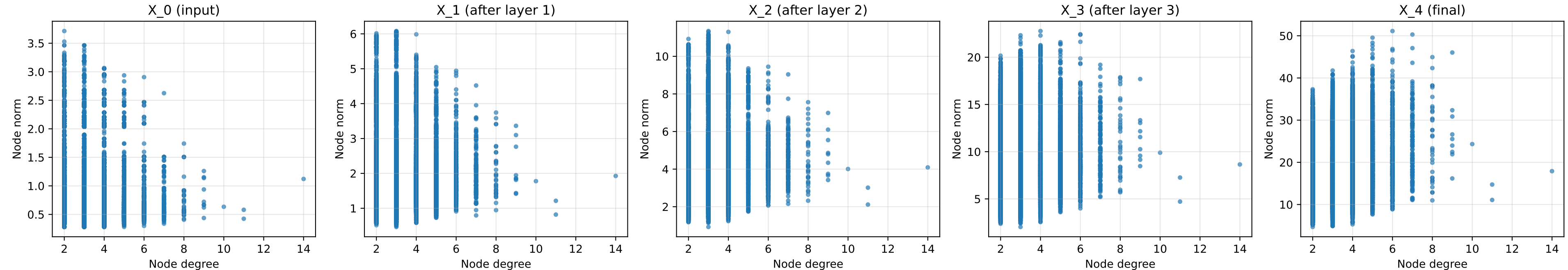
Node norm vs degree — roman_empire, JointSheafParamsAlt, stalk_dim=5
