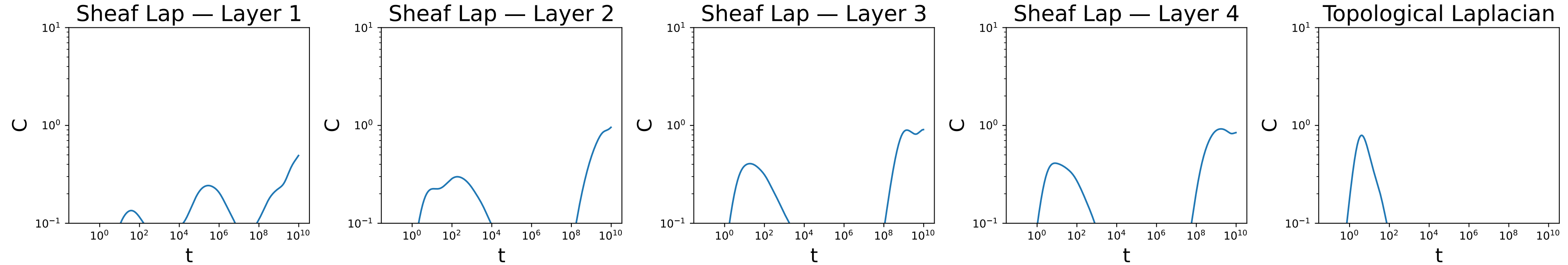
Entropic susceptibility — citeseer
