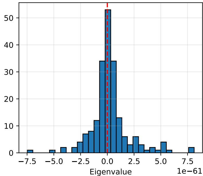
Topological Laplacian
