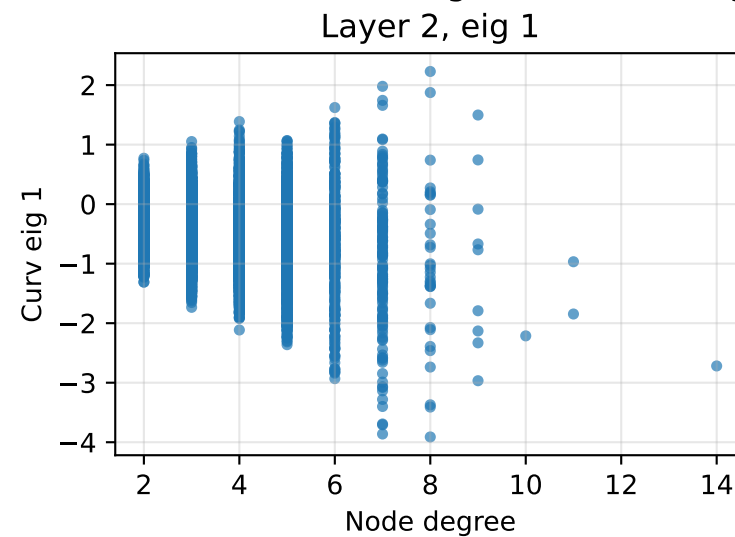
Curvature eigenvalues vs degree and topological curvature
