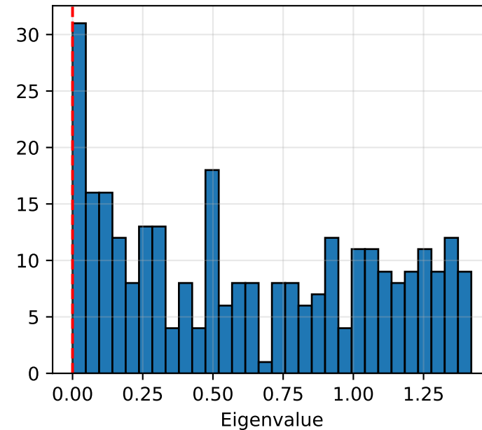
Topological Laplacian
