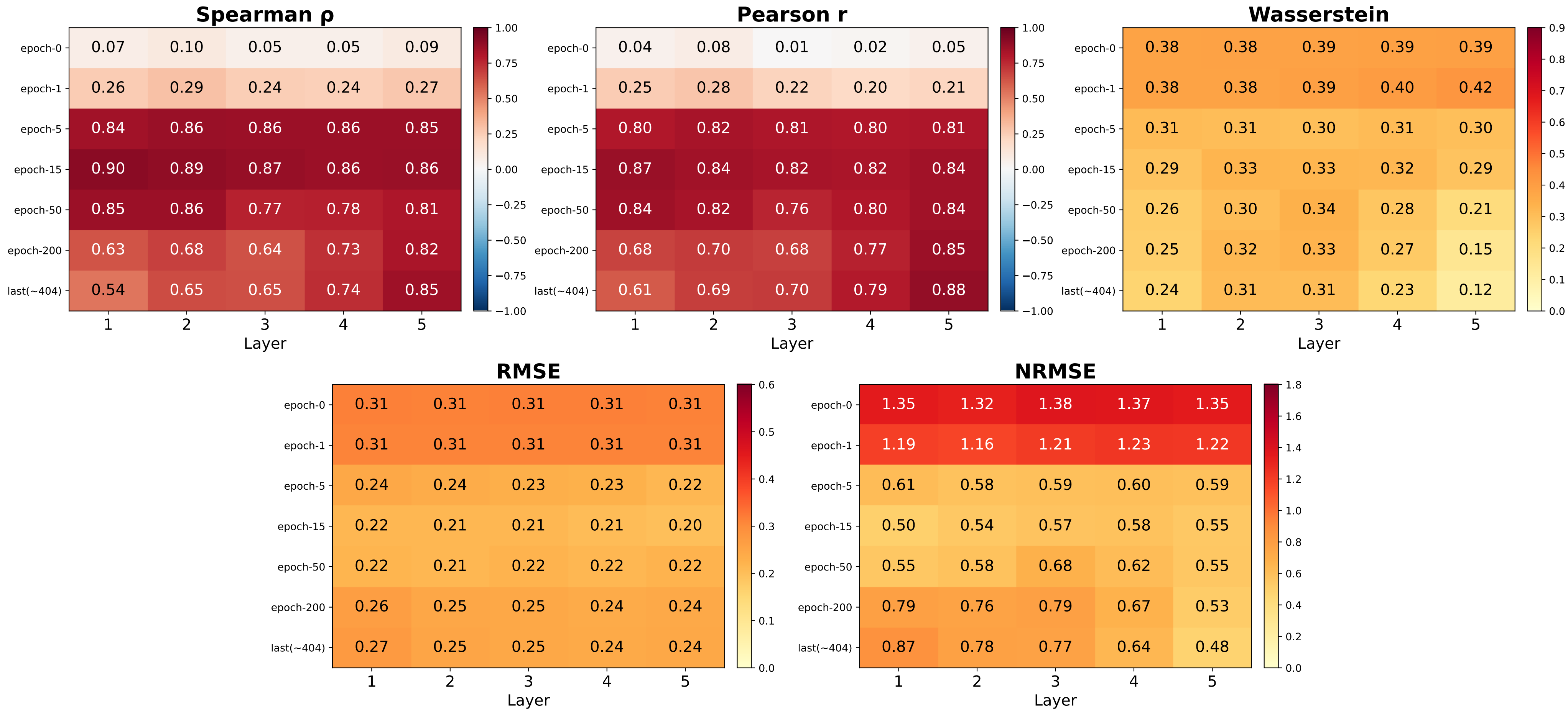
Forman Alignment Heatmap — amazon_ratings (GeneralSheaf, d=5, 5L, norm=True) (values = mean across 5 eigenvalues, averaged over folds)
