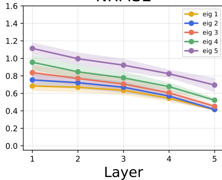
NRMSE
