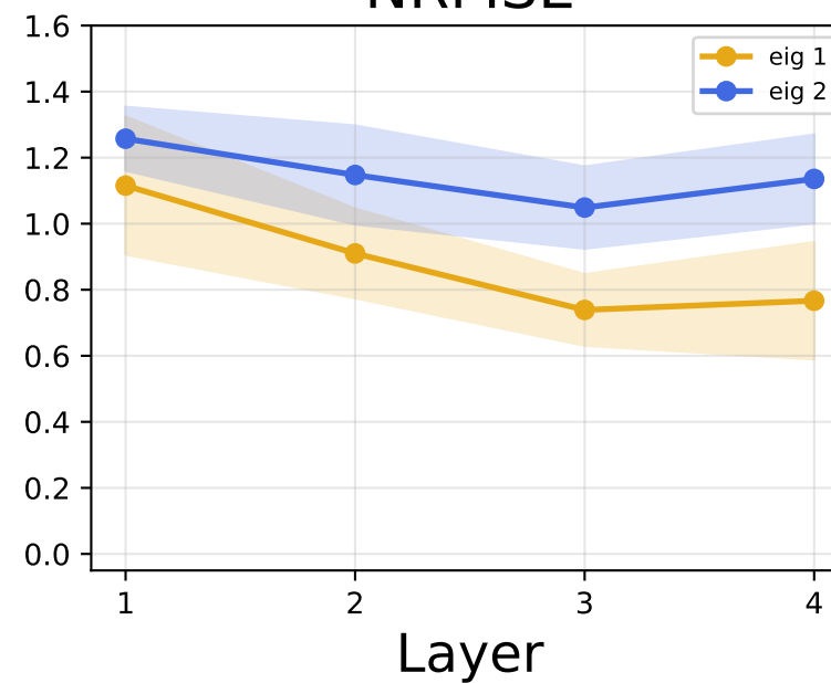
NRMSE
