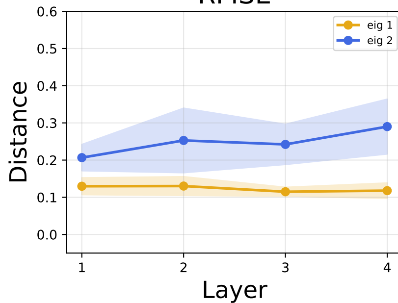
RMSE
