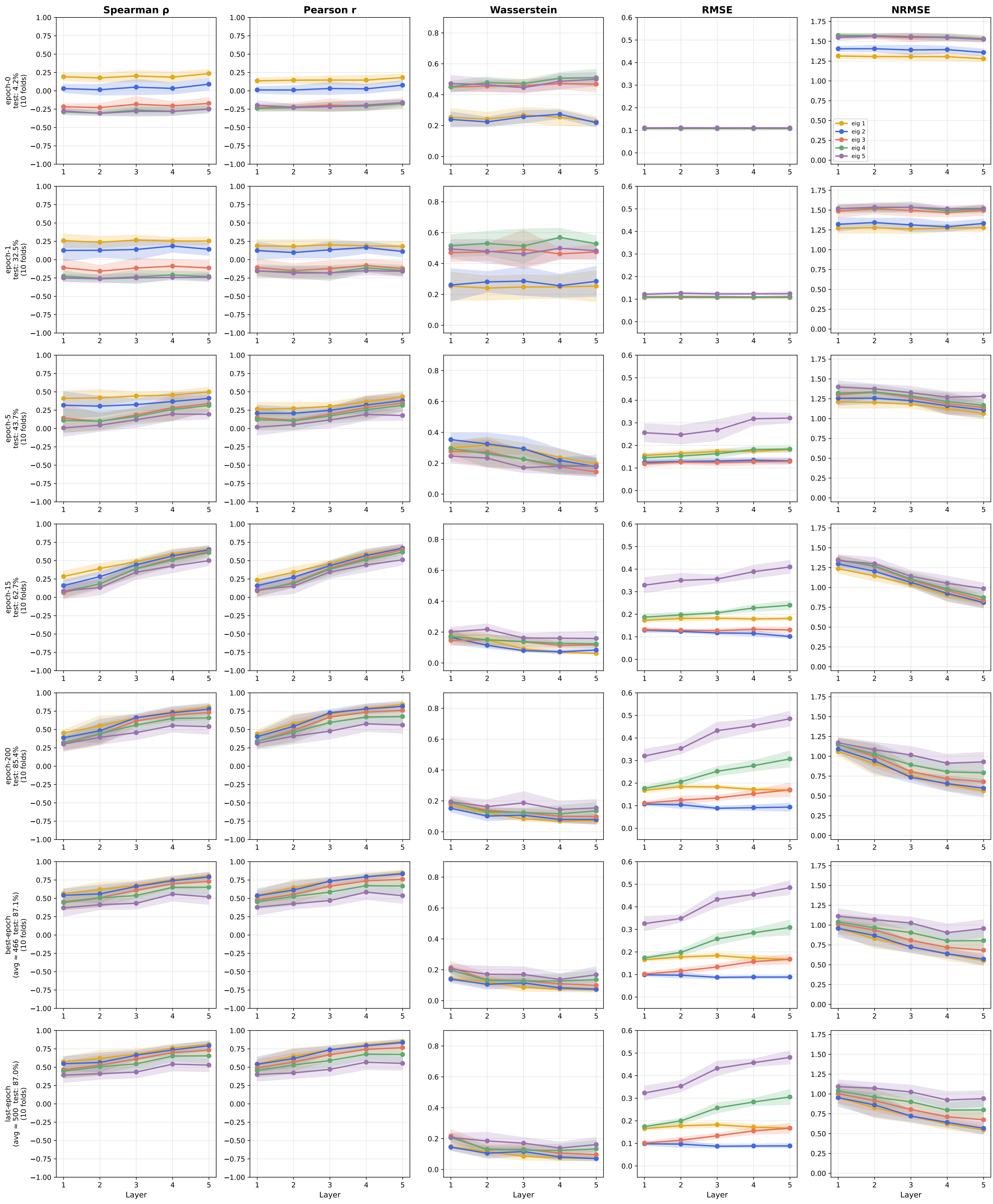
Forman Profile Evolution — roman_empire (GeneralSheaf, d=5, 5 layers)
