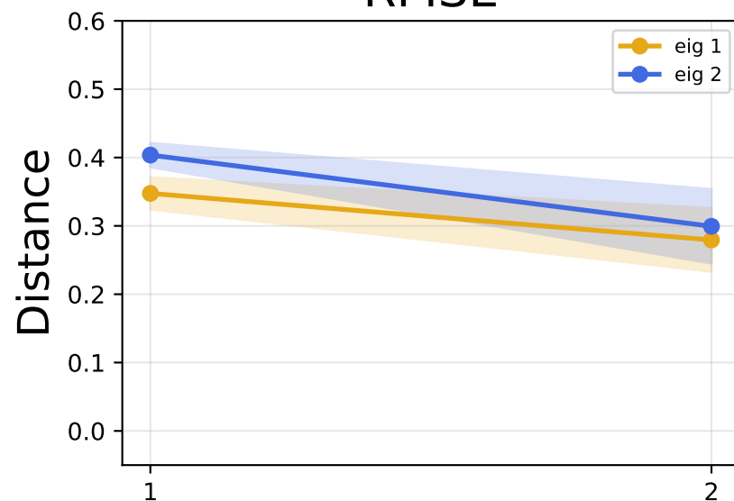
RMSE
