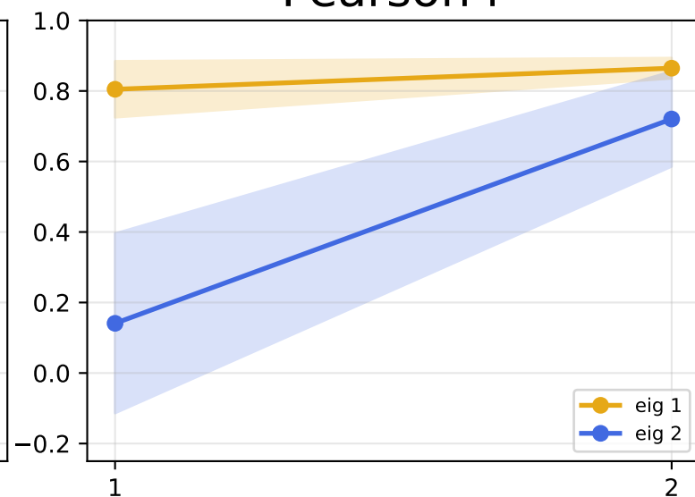
Pearson r
