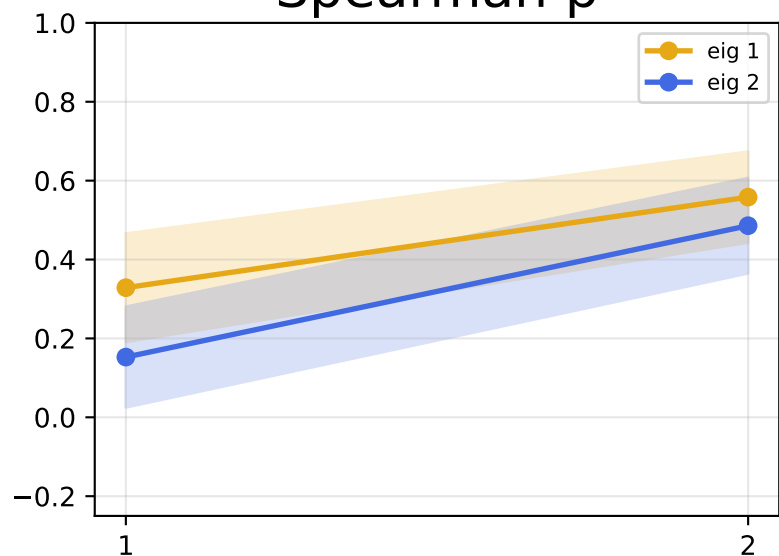
Spearman \rho
