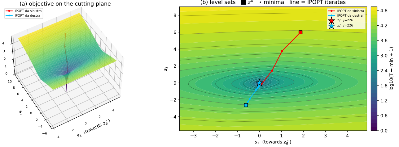
Figure 10: The objective in the decision space \mathbb{R}^{141} , on a plane constructed to contain both local minima of the recorded cycle. (a) the surface; (b) its level sets with the two minima ( \star ), the initial iterate ( \blacksquare ) and the IPOPT iterates joining them. What is plotted is not the objective f but the \ell^1 merit function T_1(z) = f(z) + \sigma \|c(z)\|_1 : in the simultaneous parametrisation X and U are independent variables tied by the dynamic equalities, so a generic point of the plane is not dynamically feasible and a plot of f alone would show a landscape the solver never traverses. The merit function is what the line search actually decreases.
