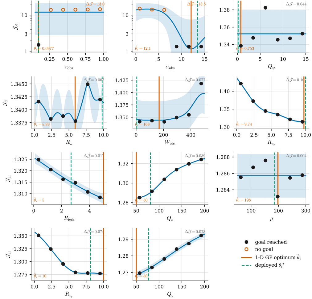
Figure 11: One-factor-at-a-time sweep: closed-loop score against each weight in turn, six rollouts and one 1-D GP per axis, with the band of (37). Filled markers reach the goal, hollow ones do not; solid line is the axis optimum (38), dashed the deployed value. \Delta\mathcal{J} , the spread of the six observations, is the only quantity comparable across panels — those containing a failure use a log axis and the rest are zoomed, so the apparent amplitude is not.
