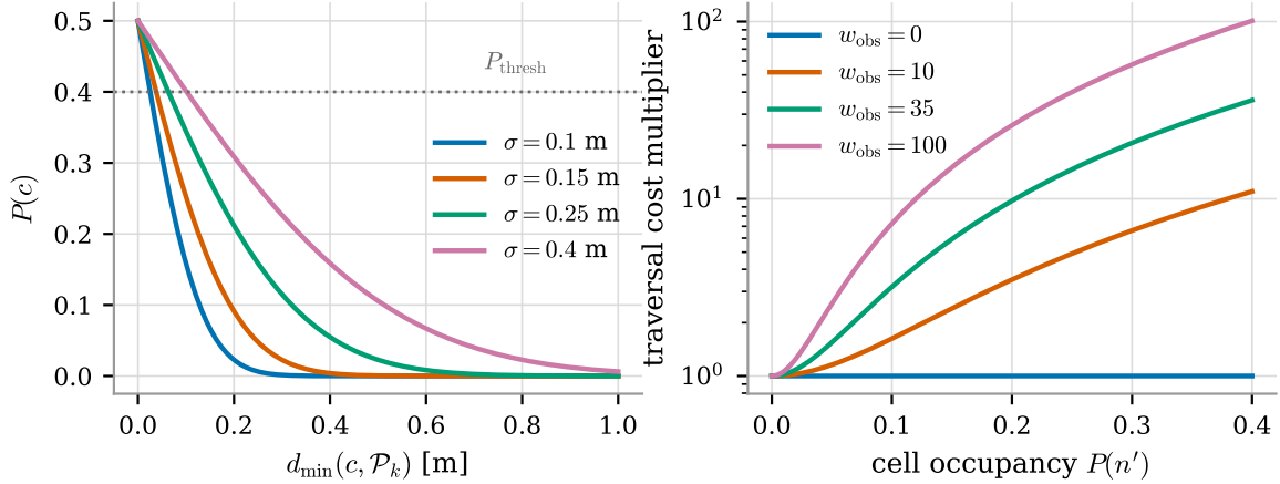
Figure 4: Left: the Gaussian inflation model (9) for four values of \sigma , with the hard threshold P_{\text{thr}} = 0.4 . Right: the soft traversal-cost multiplier 1 + w_{\text{obs}}(P/P_{\text{thr}})^2 of the A^* edge cost (15), which is what actually keeps the path away from walls; the deployed value is w_{\text{obs}} = 35 .
