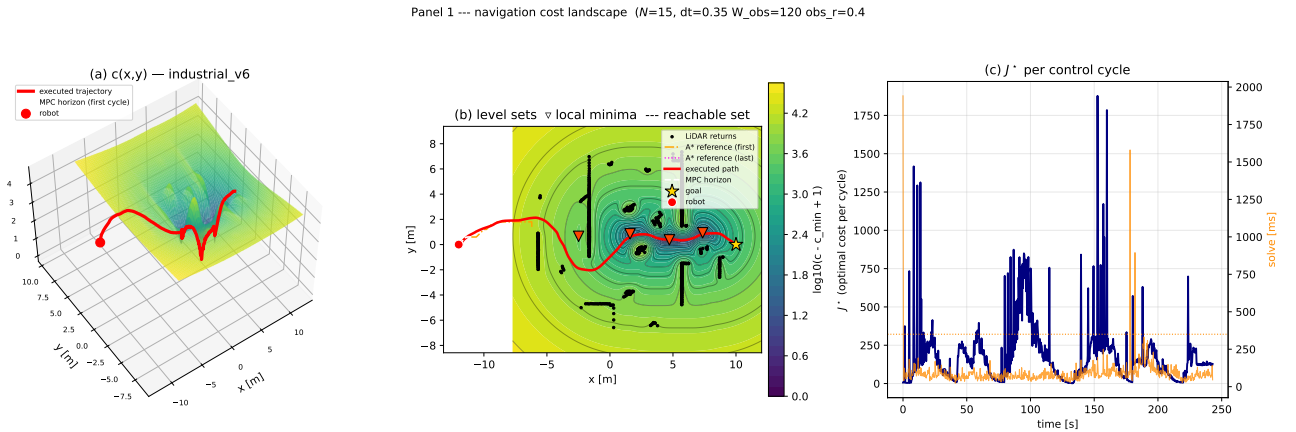
Figure 8: The navigation cost landscape of the recorded run industrial_v6 . (a) the surface c(p) of Eq. (37) over the world plane, with the executed trajectory (red) and one MPC horizon (dashed) drawn on the surface: the obstacle term raises a ridge along every wall of the plant, the tracking term forms the valley along the A^* reference. (b) the same field as level sets, with the local minima marked and the shaded region showing the set reachable within one horizon under \mathcal{U} ; the constraint, not the cost, is what excludes most of the plane. (c) the optimal cost J^* of each control cycle, and the solve time beside it. The point worth noticing is in panel (a): the trajectory does not follow steepest descent , and climbs the surface wherever doing so lowers the sum over the horizon.
