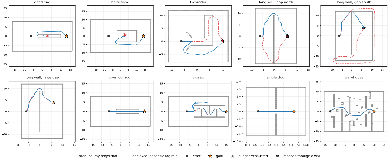
Figure 11: The ten worlds of the campaign, each with the trajectory produced by the baseline projection rule (17) (dashed) and by the deployed geodesic arg min (16) (solid), under limited perception. Heavy frames are the six traps , light frames the four controls that only look like traps. The controls are what make the result a result: a rule that simply refused to enter concave-looking scenes would pass every trap and fail all four of these, where the correct behaviour is to drive straight through. Read together with Table 14, since a trajectory that reaches the goal may have reached it through a wall.
