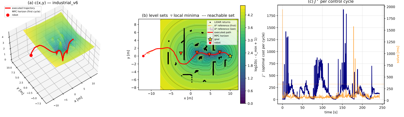
Figure 8: The navigation cost landscape of the recorded run industrial_v6 . (a) the surface c(p) of Eq. (37) over the world plane, with the executed trajectory (red) and one MPC horizon (dashed) drawn on the surface: the obstacle term raises a ridge along every wall of the plant, the tracking term forms the valley along the A^* reference. (b) the same field as level sets, with the local minima marked and the shaded region showing the set reachable within one horizon under \mathcal{U} ; the constraint, not the cost, is what excludes most of the plane. (c) the optimal cost J^* of each control cycle, and the solve time beside it. The point worth noticing is in panel (a): the trajectory does not follow steepest descent , and climbs the surface wherever doing so lowers the sum over the horizon.
