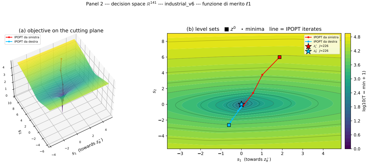
Figure 10: The objective in the decision space \mathbb{R}^{141} , on a plane constructed to contain both local minima of the recorded cycle. (a) the surface; (b) its level sets with the two minima ( \star ), the initial iterate ( \blacksquare ) and the IPOPT iterates joining them. What is plotted is not the objective f but the \ell^1 merit function T_1(z) = f(z) + \sigma \|c(z)\|_1 : in the simultaneous parametrisation X and U are independent variables tied by the dynamic equalities, so a generic point of the plane is not dynamically feasible and a plot of f alone would show a landscape the solver never traverses. The merit function is what the line search actually decreases.
