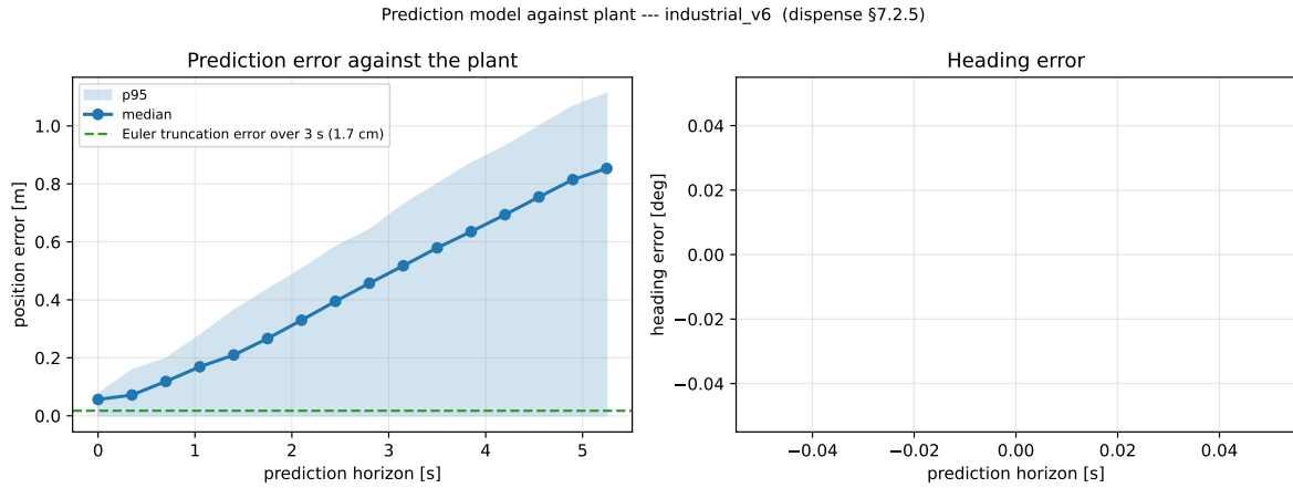
Figure 8: Prediction error against the position along the horizon, over 695 cycles of the recorded run industrial_v6 : median and 95th percentile. The residual at k = 0 is time misalignment between the instant the prediction is published and the instant the pose is sampled, not model error, and is subtracted before quoting the divergence.
