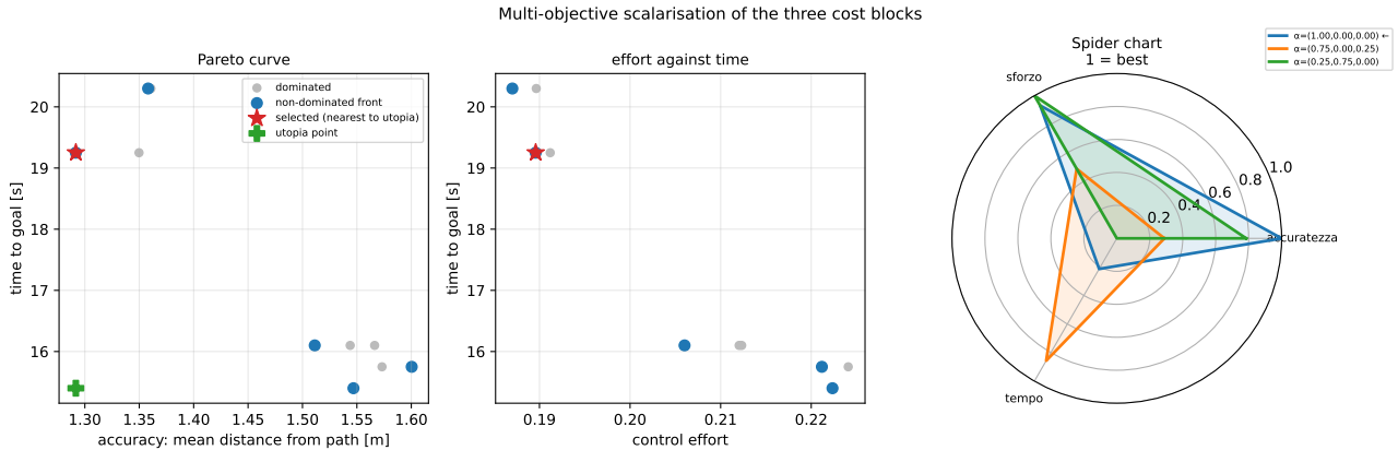
Figure 12: Sampling of the weight simplex: the achieved objectives for each scalarisation, the non-dominated set, and the utopia point. The metrics used to evaluate the solutions use fixed weights, not the sampled ones — otherwise each point of the simplex would be judged by a different yardstick.
