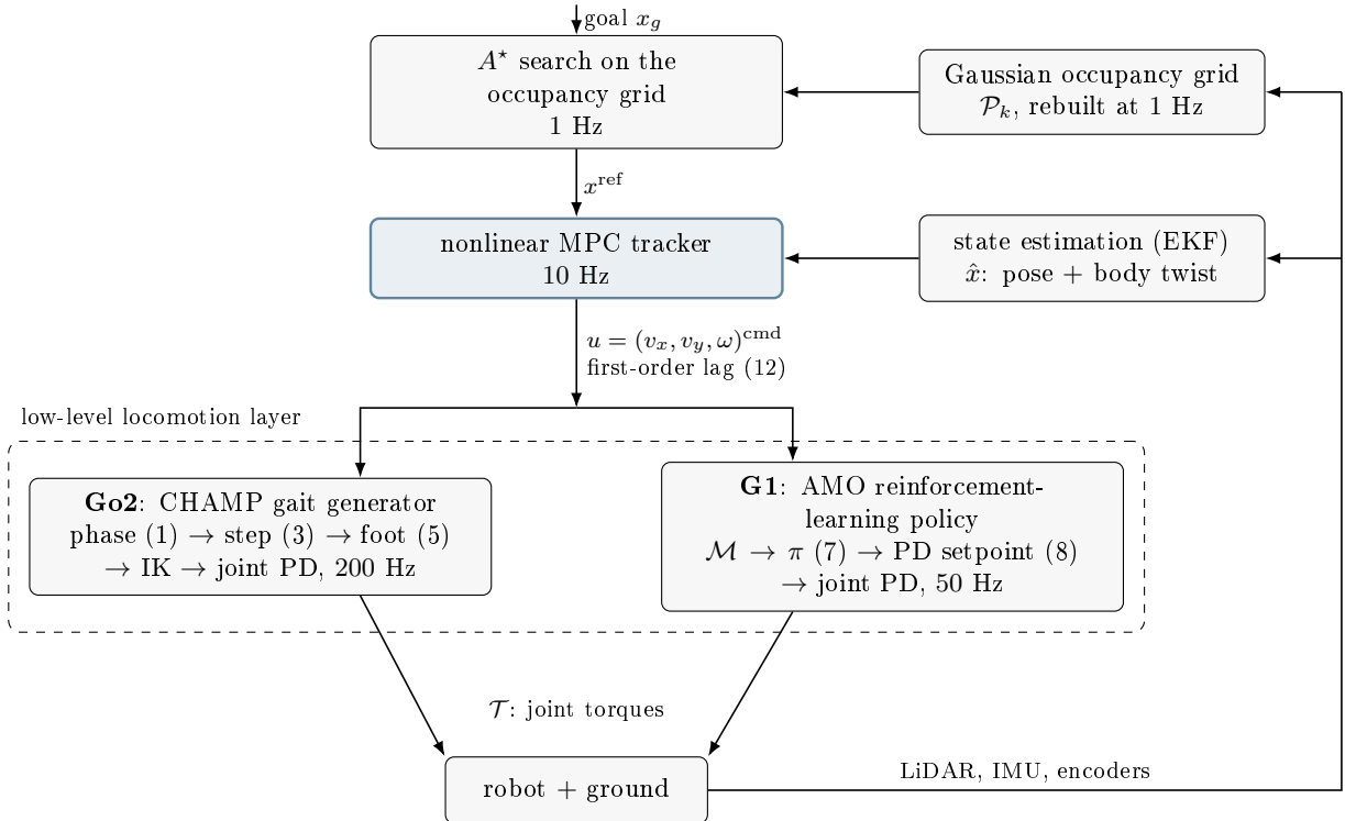
Figure 3: Cascaded structure of the controller, from the goal down to joint torques. The rates fall by roughly a decade at every seam (1 Hz, 10 Hz, 50–200 Hz, motor-driver rate), which is what allows the layers to be designed separately, and the two branches inside the dashed box, a hand-designed gait generator and a learned policy, are interchangeable precisely because they present the same twist interface u .
