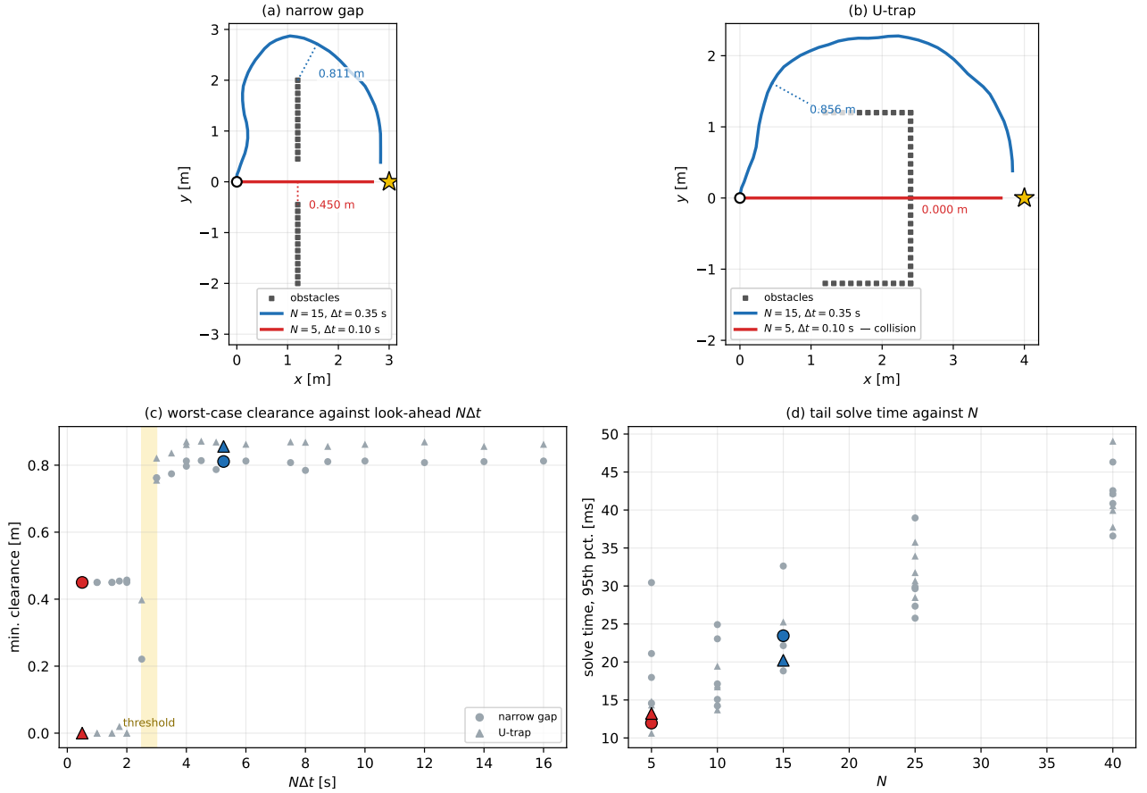
Figure 10: The deployed configuration against the cheapest one the campaign returns. (a), (b) the executed trajectories in the two worlds, with the point of minimum clearance marked. At N = 15 , \Delta t = 0.35 s the controller routes around the obstacle in both; at N = 5 , \Delta t = 0.10 s it drives straight at the goal, which in narrow gap means taking the gap down its centreline and in U-trap means passing through the back wall. (c) minimum clearance against the look-ahead N\Delta t for all 50 runs of the campaign: the transition is between 2.5 and 3 s and it does not depend on which (N, \Delta t) pair realises the look-ahead. (d) the tail solve time against N , the only parameter that governs it. The two highlighted configurations are the same in all four panels.
