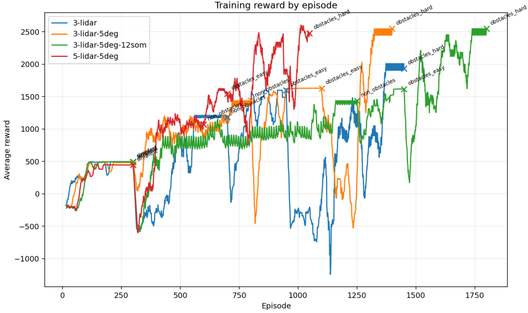
Figure 4: Moving average of training reward by episode.
