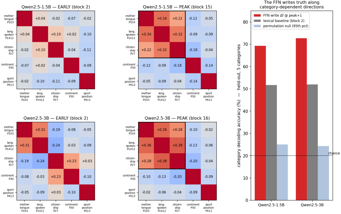
Figure 3: The category geometry: early vs. peak signed-cosine matrices, and decoding vs. the lexical baseline.
