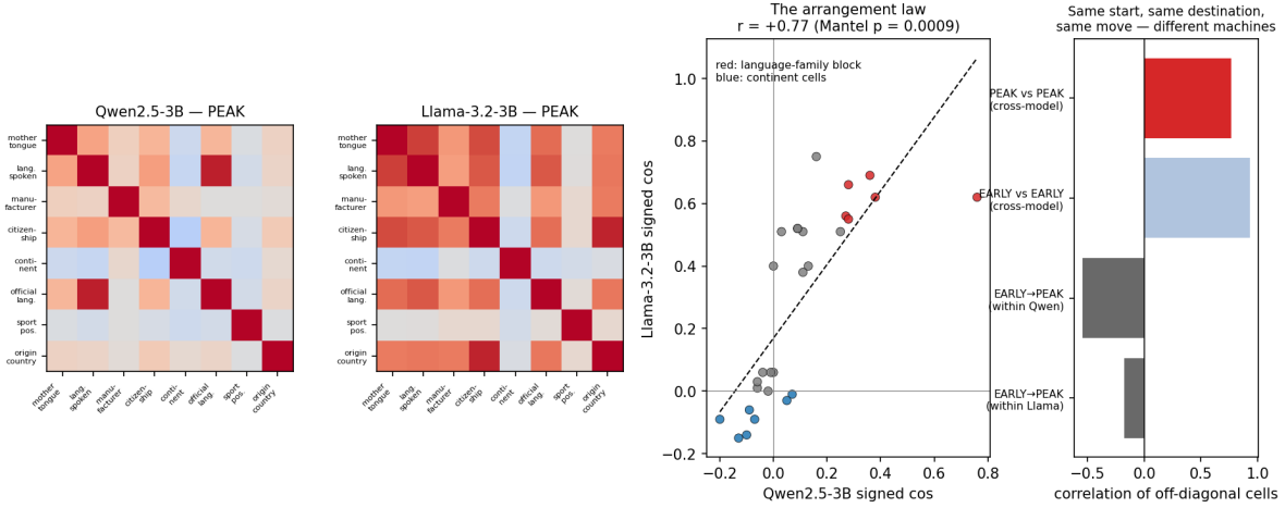
Figure 4: The arrangement law (R5). Left: the two K=8 peak signed-cosine matrices. Center: their off-diagonal cells against each other. Right: cross-model agreement at the peak and at the embedding level, and the within-model reorganization between them.
