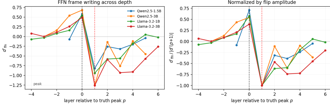
Figure 1: The FFN’s frame writing ( d' ) across depth, aligned at the truth peak, four models. Right: normalized by the flip amplitude.
