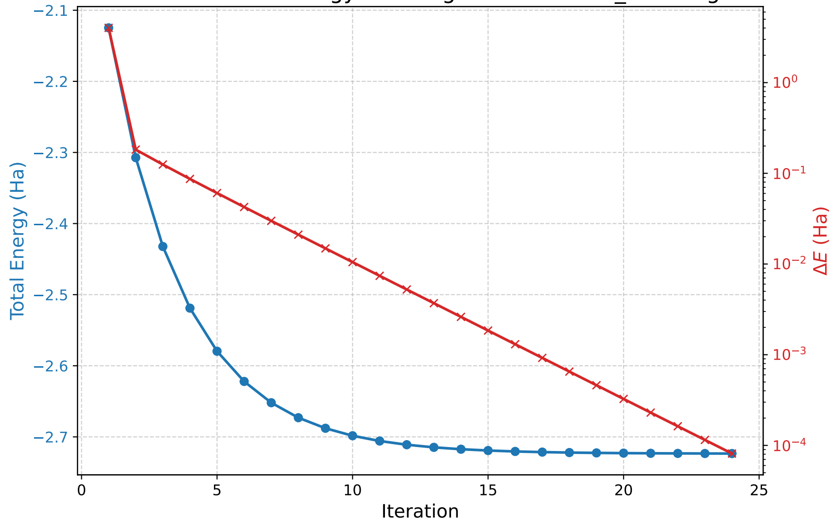
Self-Consistent Energy Convergence - Hartree_Exchange
