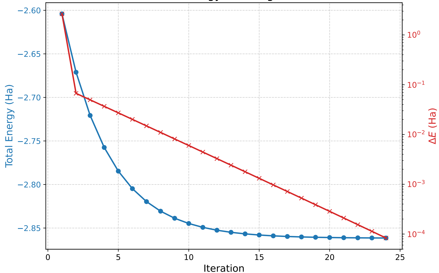
Self-Consistent Energy Convergence - Hartree
